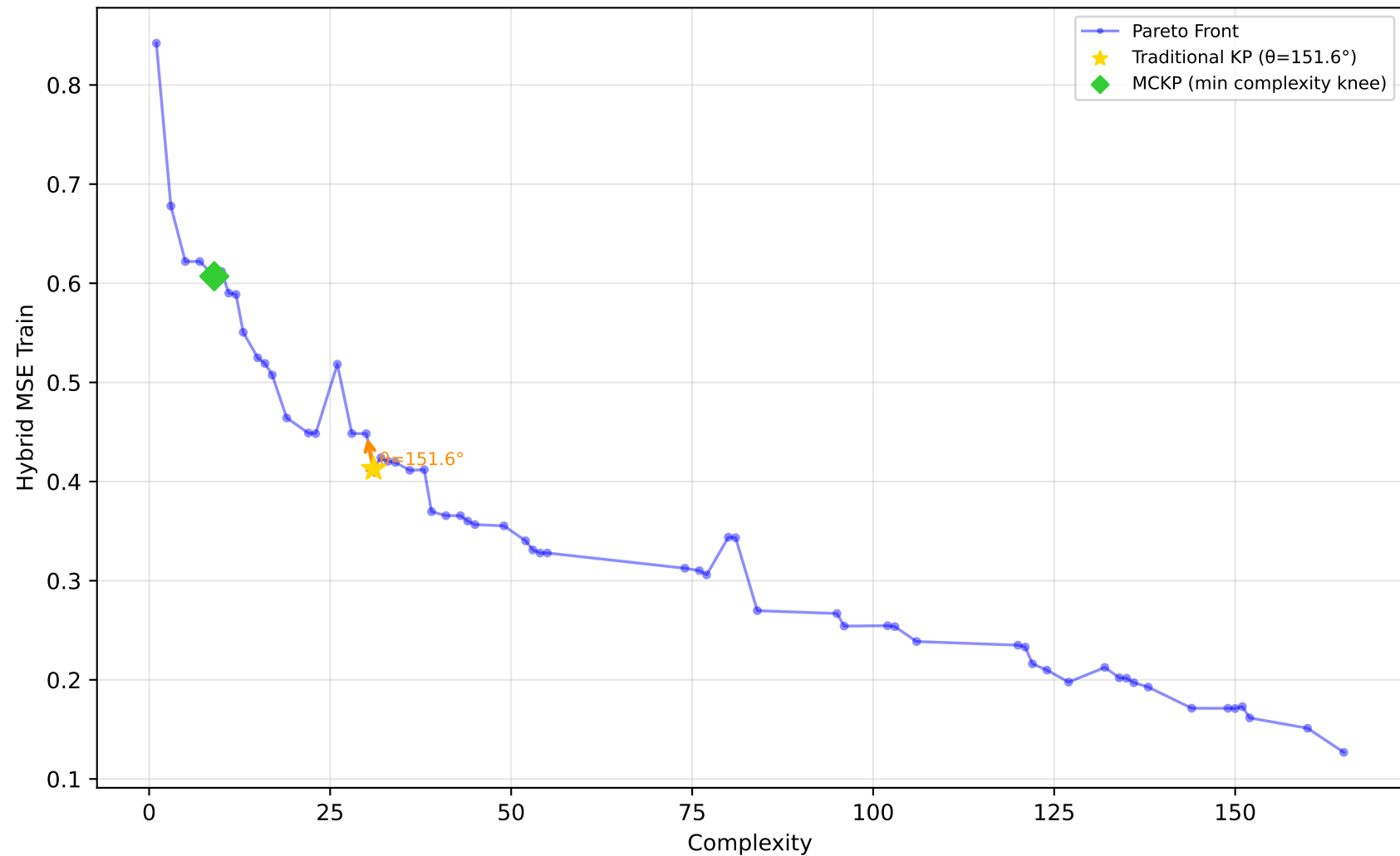
678_visualizing_environmental - Run 6 - SVP - Hybrid MSE Train \lambda_1=0.40, \lambda_2=0.00, \lambda_3=0.00 | Difficulty: 0.72 | Method: hmr
