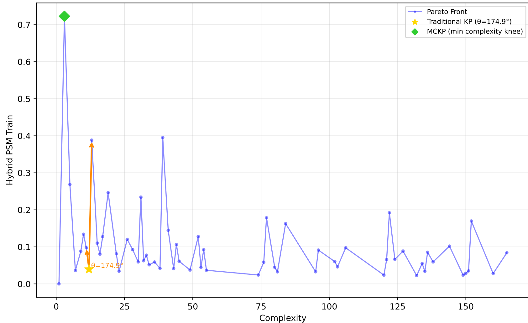
678_visualizing_environmental - Run 6 - SVP - Hybrid PSM Train \lambda_1=0.40, \lambda_2=0.00, \lambda_3=0.00 | Difficulty: 0.72 | Method: hmr
