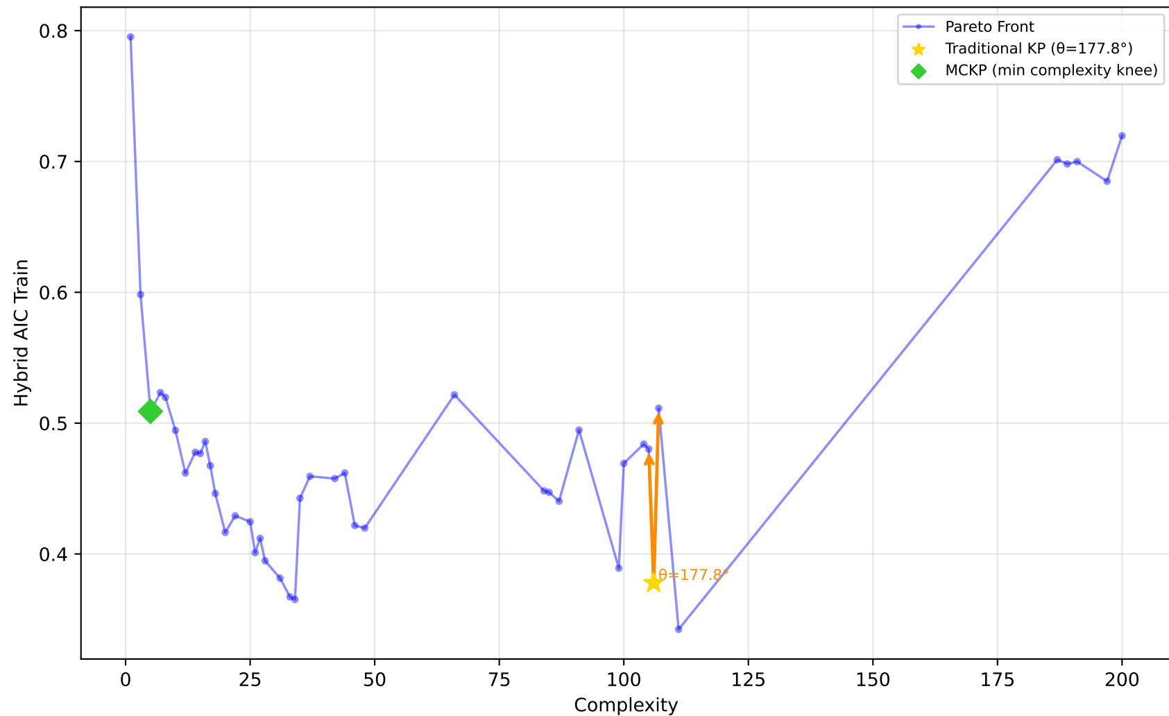
678_visualizing_environmental - Run 7 - MVP - Hybrid AIC Train \lambda_1=0.00, \lambda_2=0.00, \lambda_3=0.10 | Difficulty: 0.57 | Method: mckp
