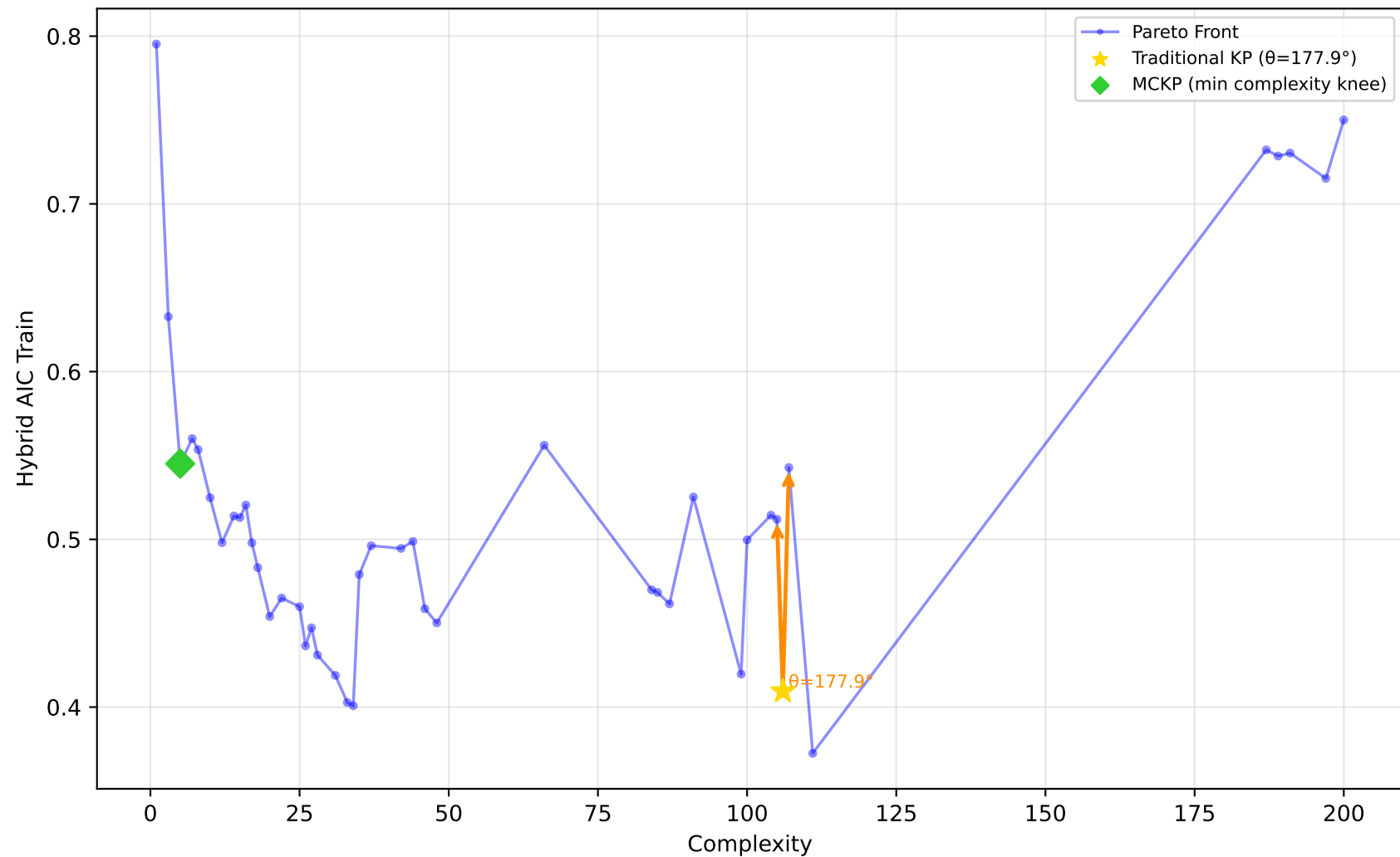
678_visualizing_environmental - Run 7 - MVP - Hybrid AIC Train \lambda_1=0.40, \lambda_2=0.00, \lambda_3=0.00 | Difficulty: 0.57 | Method: mckp
