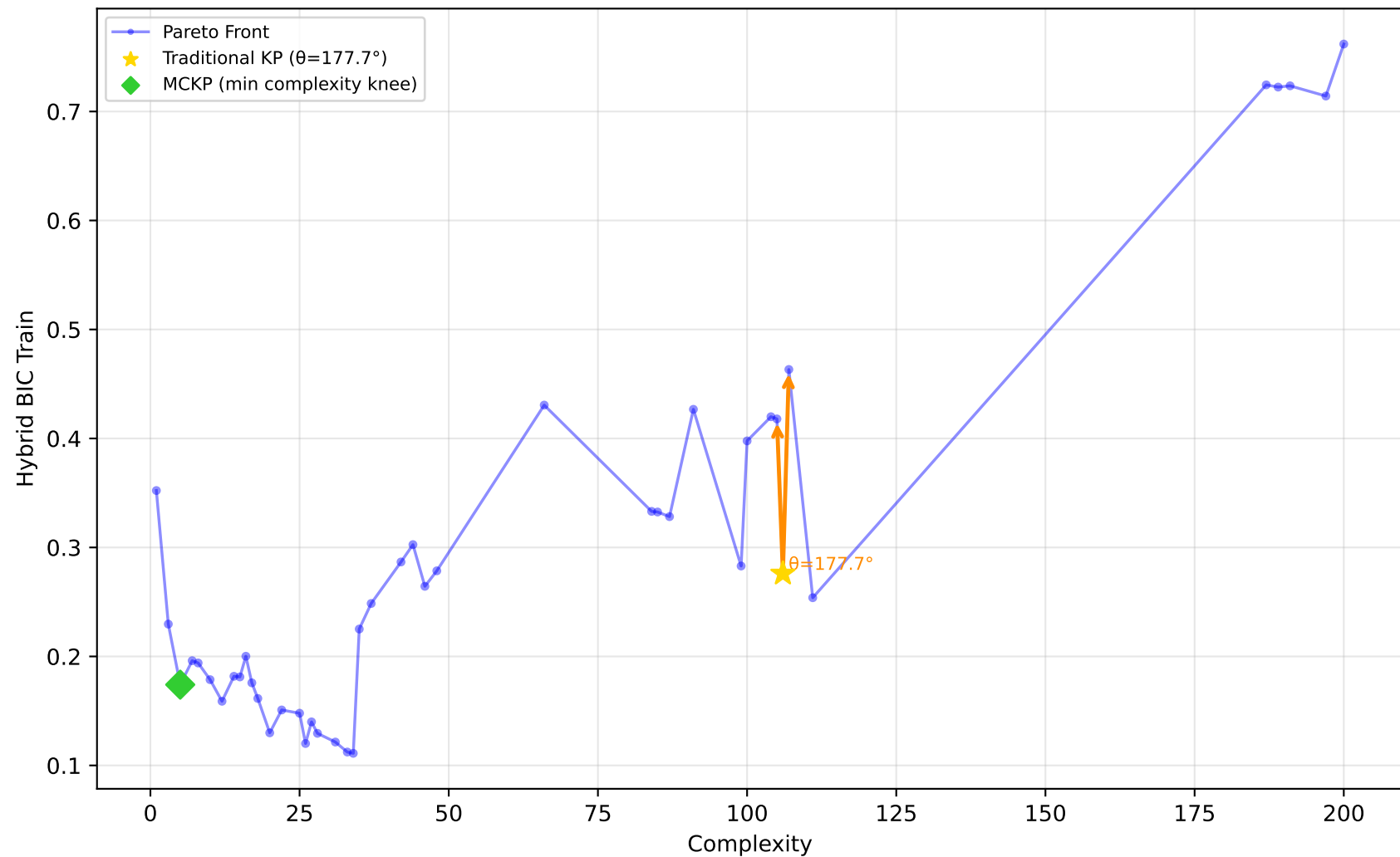
678_visualizing_environmental - Run 7 - MVP - Hybrid BIC Train \lambda_1=0.00, \lambda_2=0.00, \lambda_3=0.10 | Difficulty: 0.57 | Method: mckp
