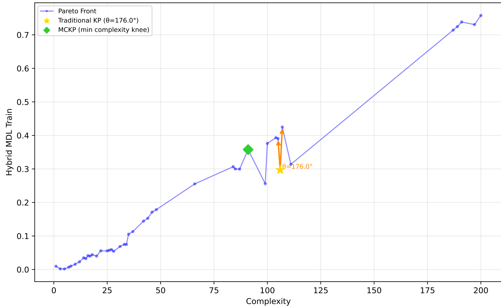
678_visualizing_environmental - Run 7 - MVP - Hybrid MDL Train \lambda_1=0.00, \lambda_2=0.00, \lambda_3=0.10 | Difficulty: 0.57 | Method: mckp
