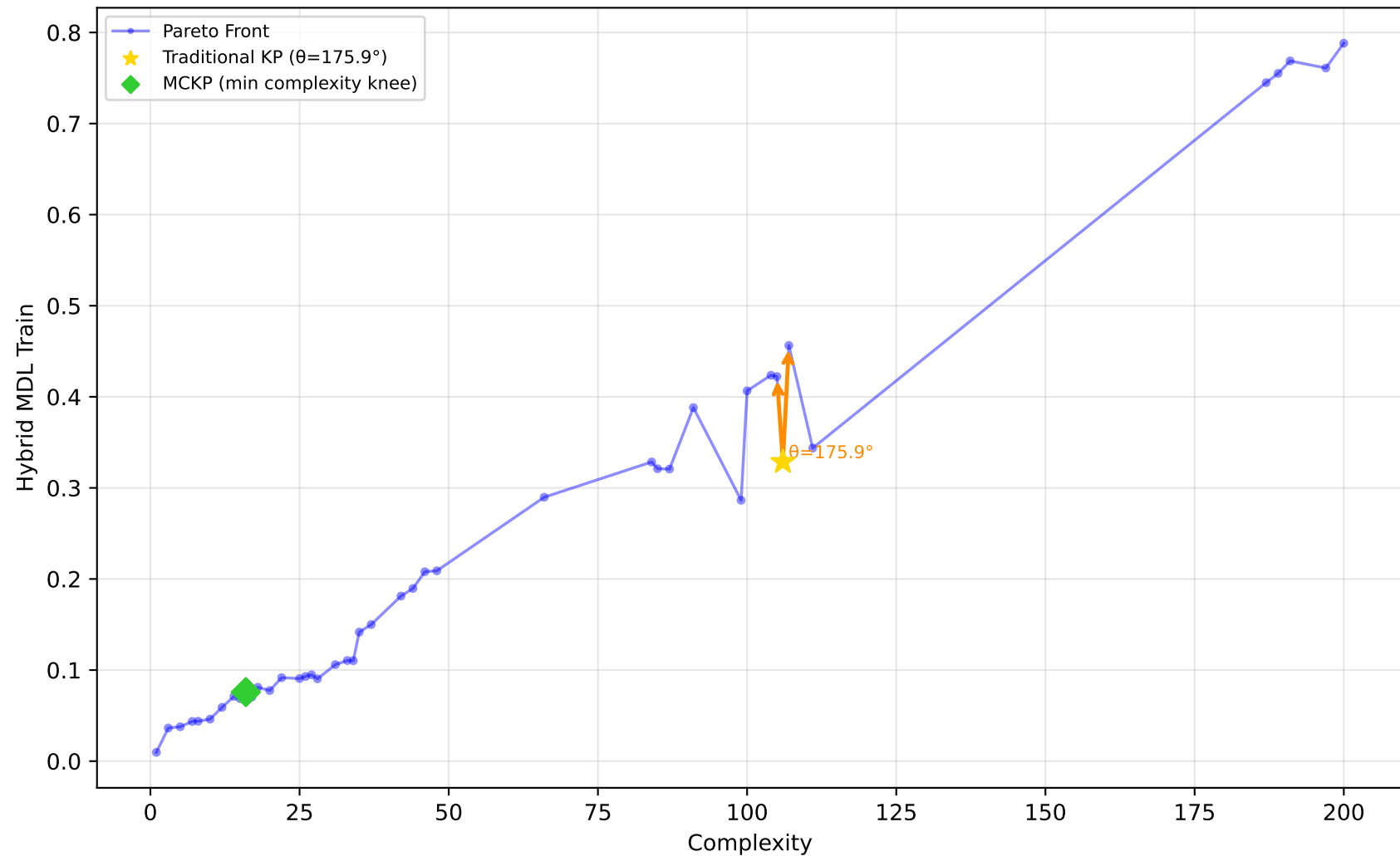
678_visualizing_environmental - Run 7 - MVP - Hybrid MDL Train \lambda_1=0.40, \lambda_2=0.00, \lambda_3=0.00 | Difficulty: 0.57 | Method: mckp
