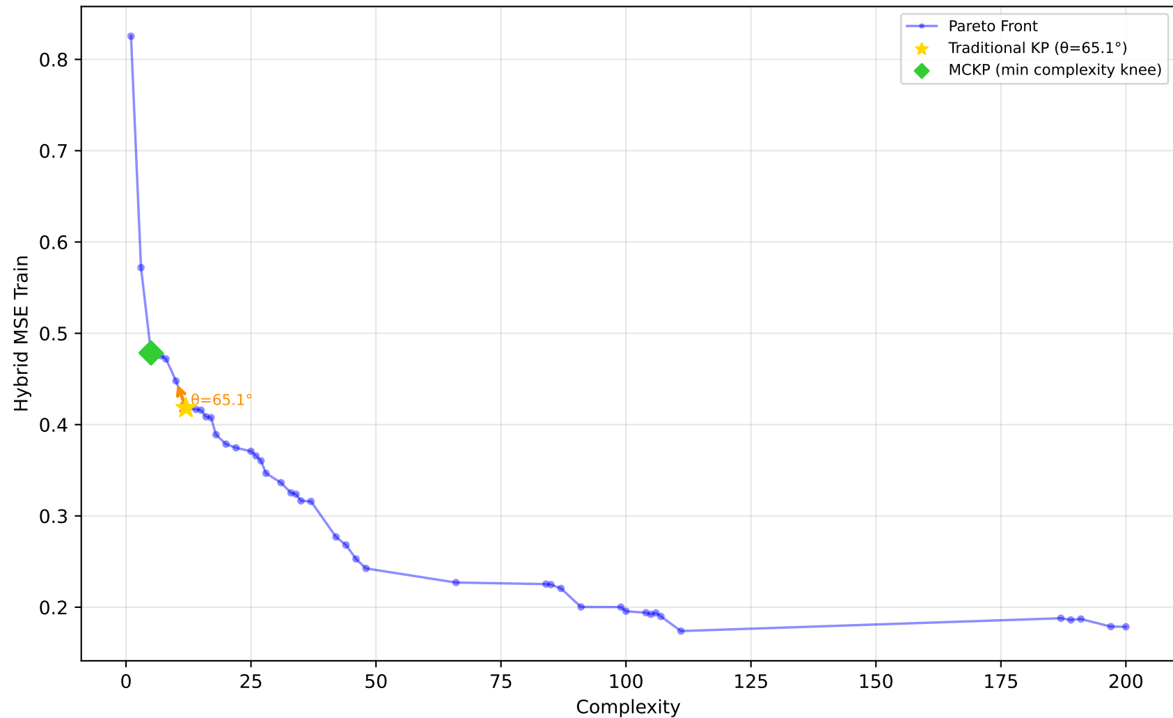
678_visualizing_environmental - Run 7 - MVP - Hybrid MSE Train \lambda_1=0.00, \lambda_2=0.00, \lambda_3=0.10 | Difficulty: 0.57 | Method: mckp
