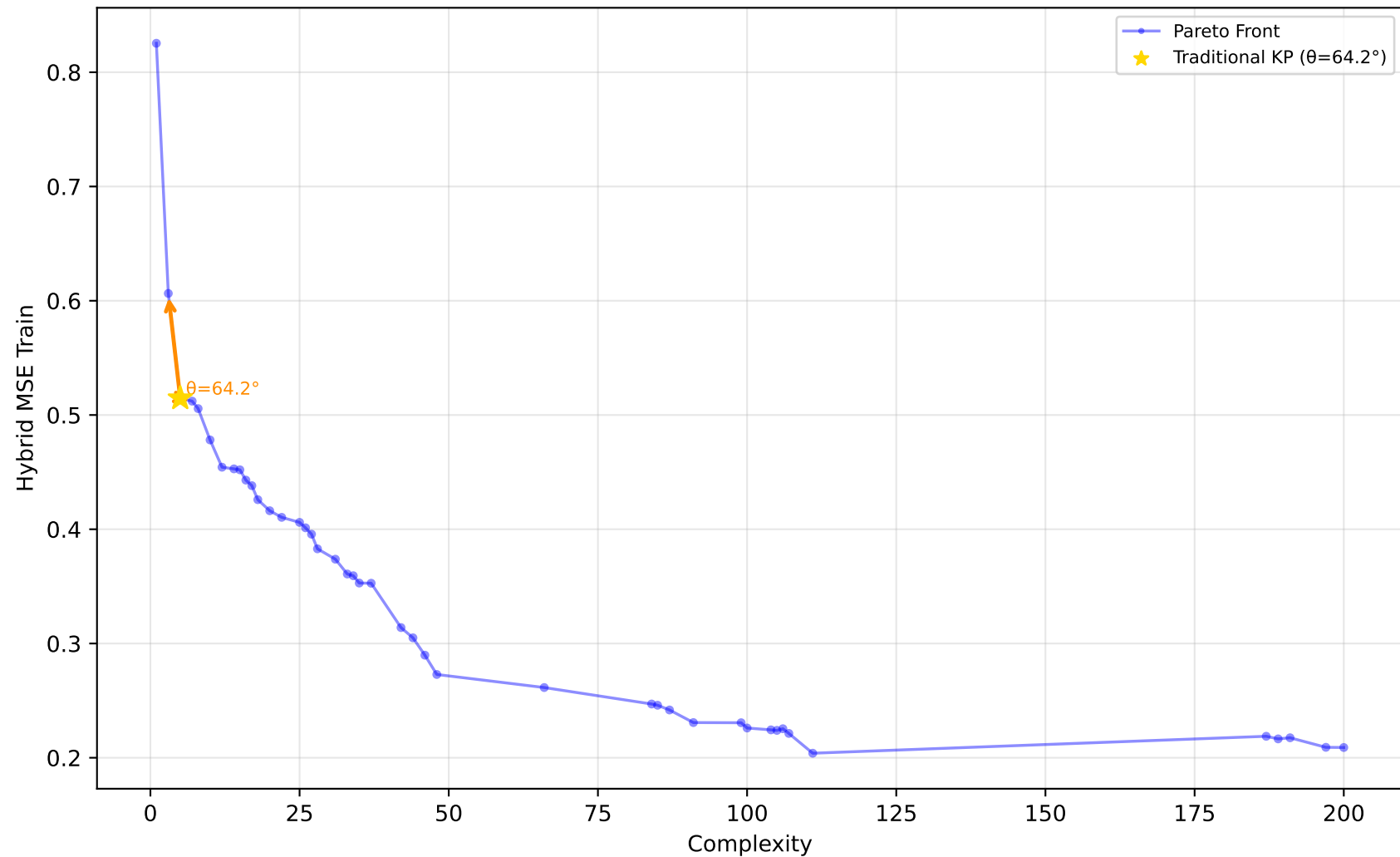
678_visualizing_environmental - Run 7 - MVP - Hybrid MSE Train \lambda_1=0.40, \lambda_2=0.00, \lambda_3=0.00 | Difficulty: 0.57 | Method: mckp
