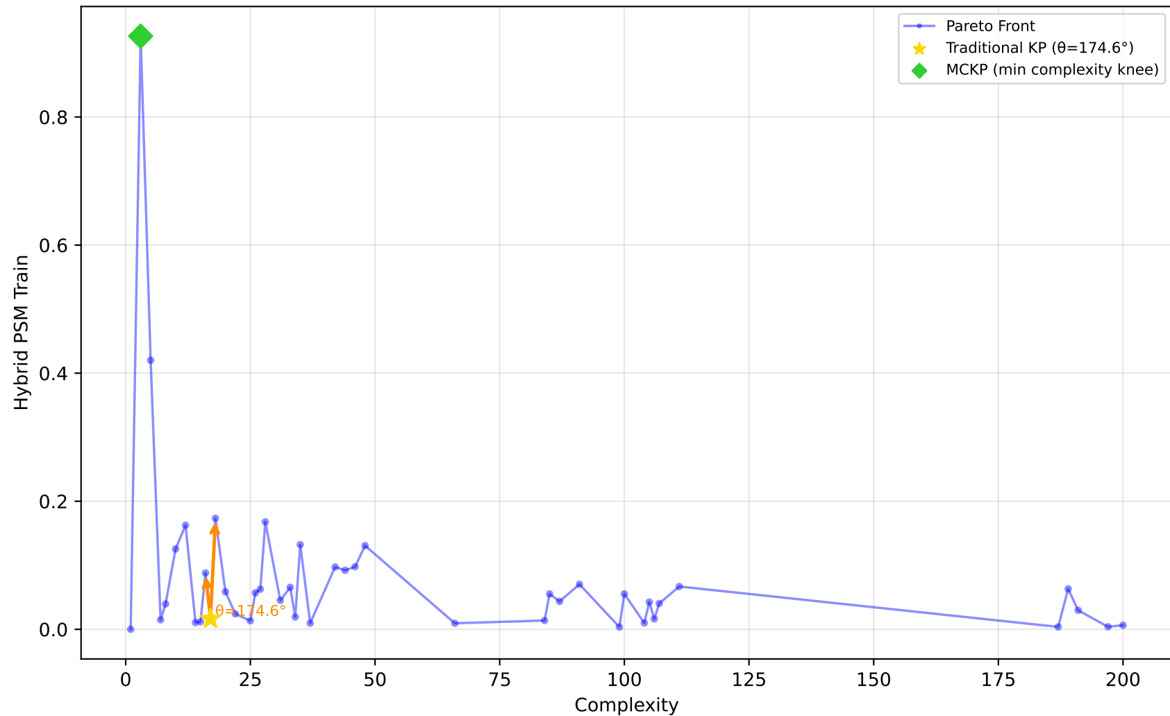
678_visualizing_environmental - Run 7 - MVP - Hybrid PSM Train \lambda_1=0.00, \lambda_2=0.00, \lambda_3=0.10 | Difficulty: 0.57 | Method: mckp
