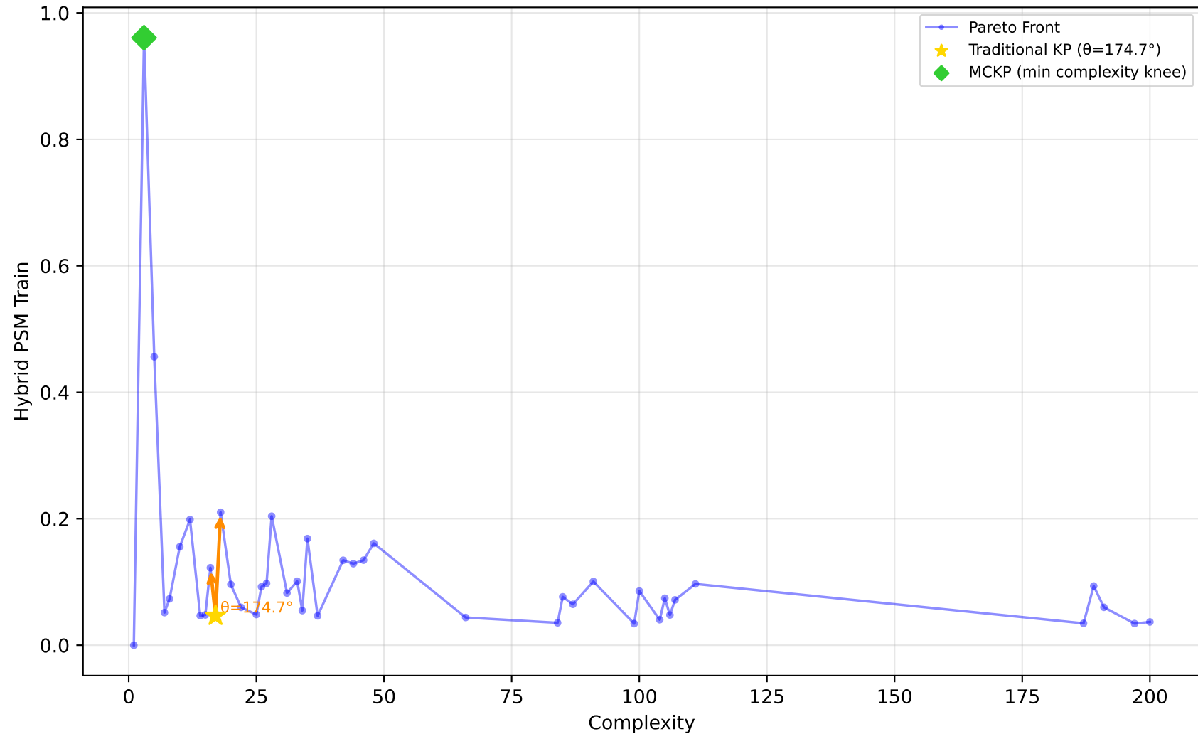
678_visualizing_environmental - Run 7 - MVP - Hybrid PSM Train \lambda_1=0.40, \lambda_2=0.00, \lambda_3=0.00 | Difficulty: 0.57 | Method: mckp
