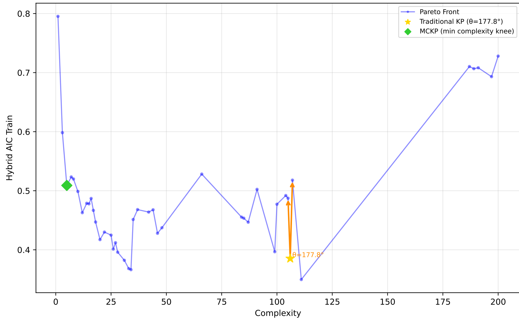
678_visualizing_environmental - Run 7 - SVP - Hybrid AIC Train \lambda_1=0.00, \lambda_2=0.10, \lambda_3=0.20 | Difficulty: 0.57 | Method: mckp
