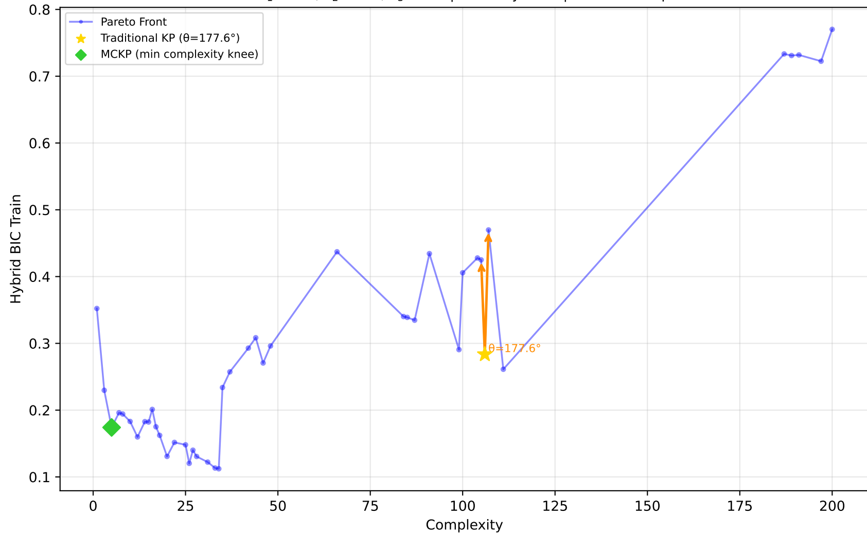
678_visualizing_environmental - Run 7 - SVP - Hybrid BIC Train \lambda_1=0.00, \lambda_2=0.10, \lambda_3=0.20 | Difficulty: 0.57 | Method: mckp
