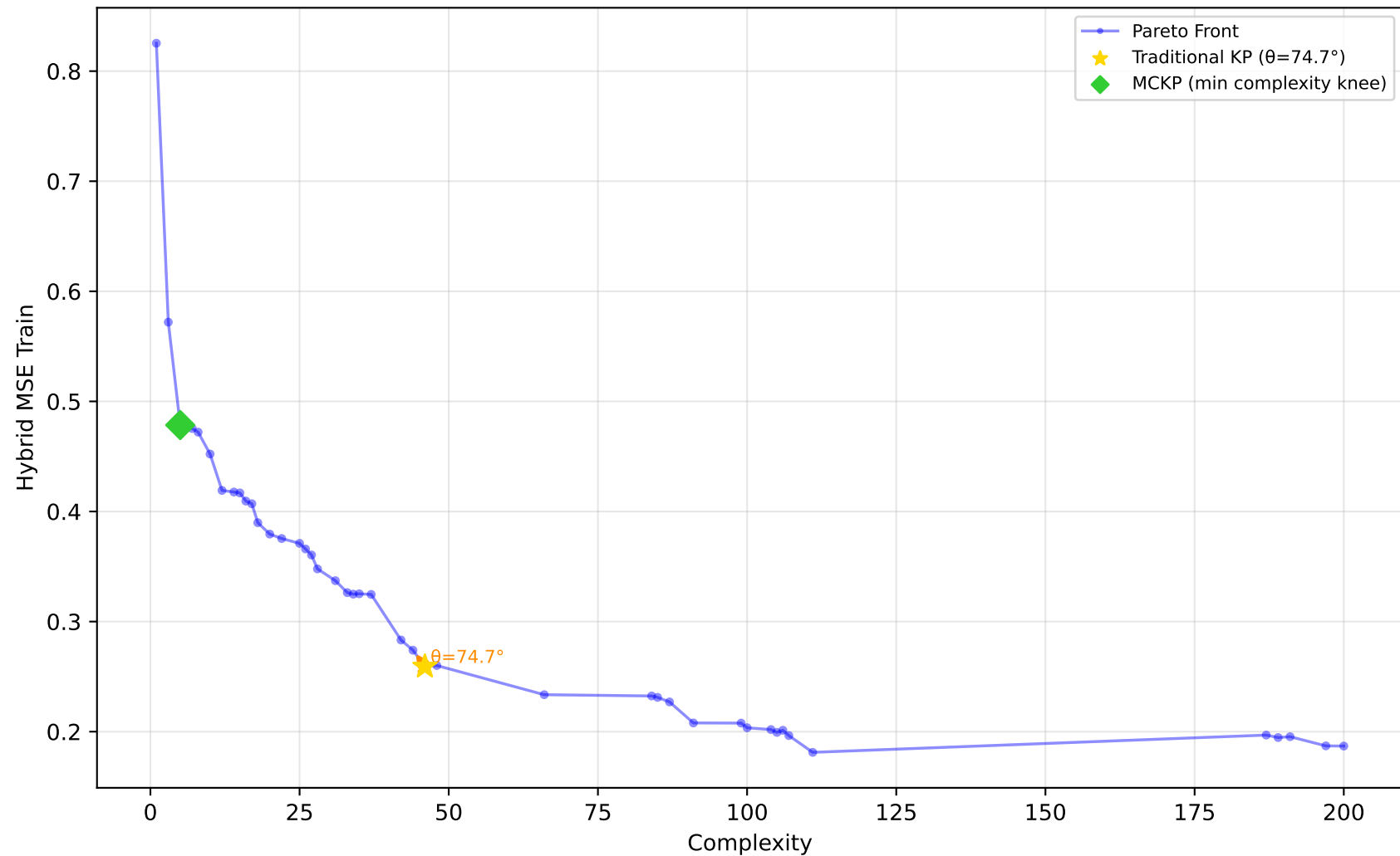
678_visualizing_environmental - Run 7 - SVP - Hybrid MSE Train \lambda_1=0.00 , \lambda_2=0.10 , \lambda_3=0.20 | Difficulty: 0.57 | Method: mckp
