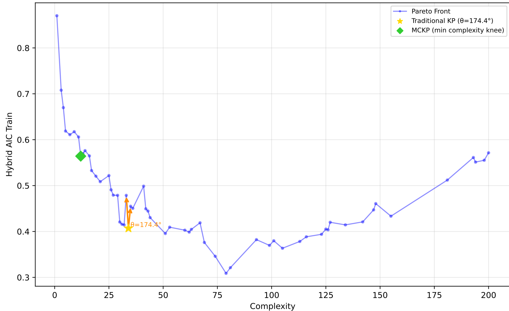
678_visualizing_environmental - Run 8 - MVP - Hybrid AIC Train \lambda_1=0.00, \lambda_2=0.00, \lambda_3=0.10 | Difficulty: 0.21 | Method: mckp
