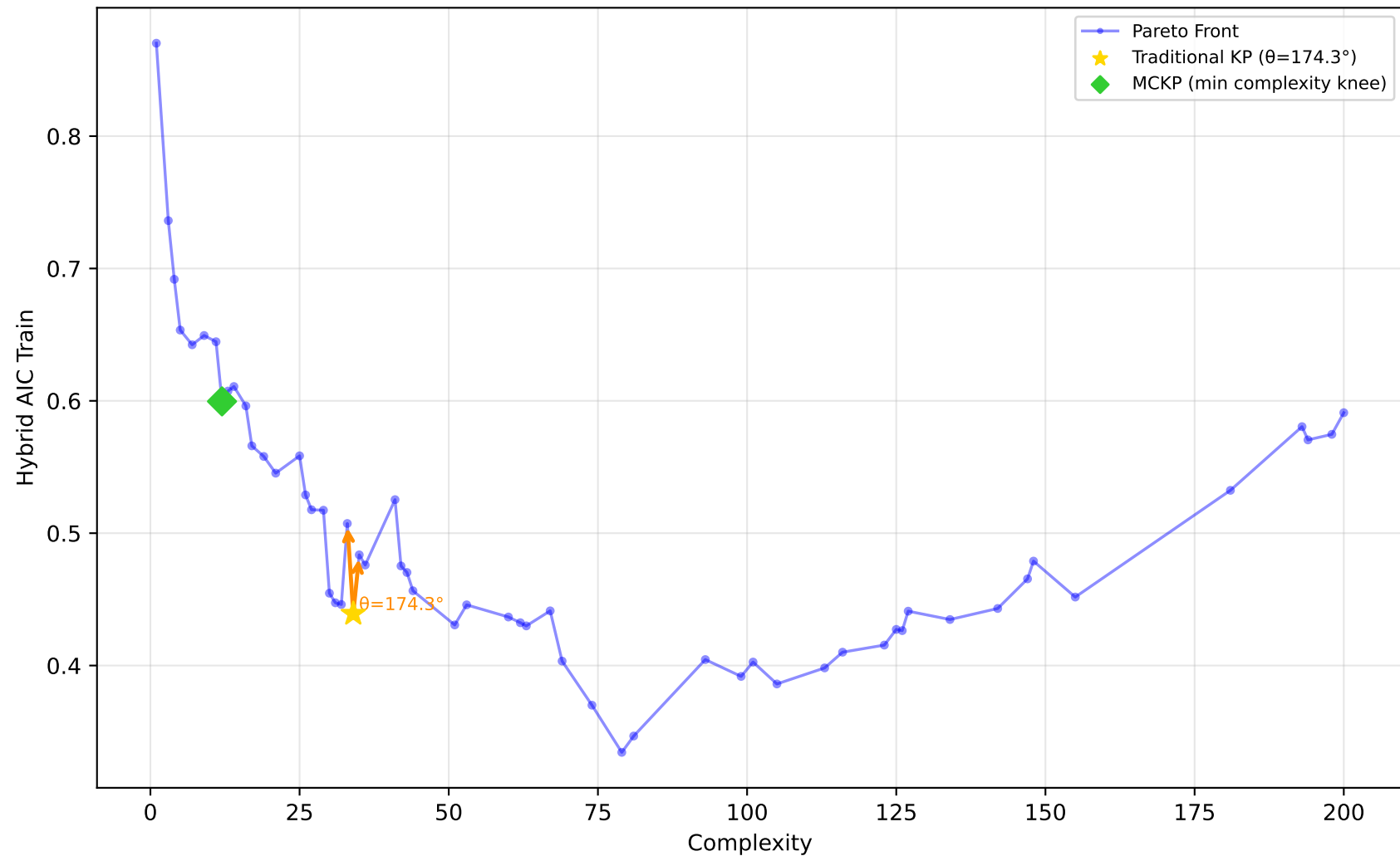
678_visualizing_environmental - Run 8 - MVP - Hybrid AIC Train \lambda_1=0.40, \lambda_2=0.00, \lambda_3=0.00 | Difficulty: 0.21 | Method: mckp
