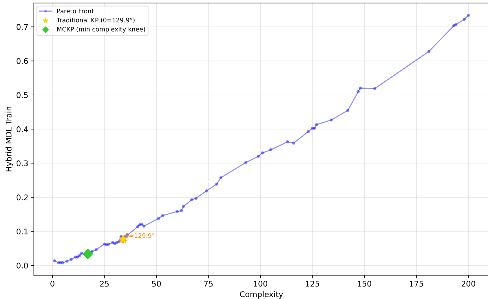
678_visualizing_environmental - Run 8 - MVP - Hybrid MDL Train \lambda_1=0.00, \lambda_2=0.00, \lambda_3=0.10 | Difficulty: 0.21 | Method: mckp
