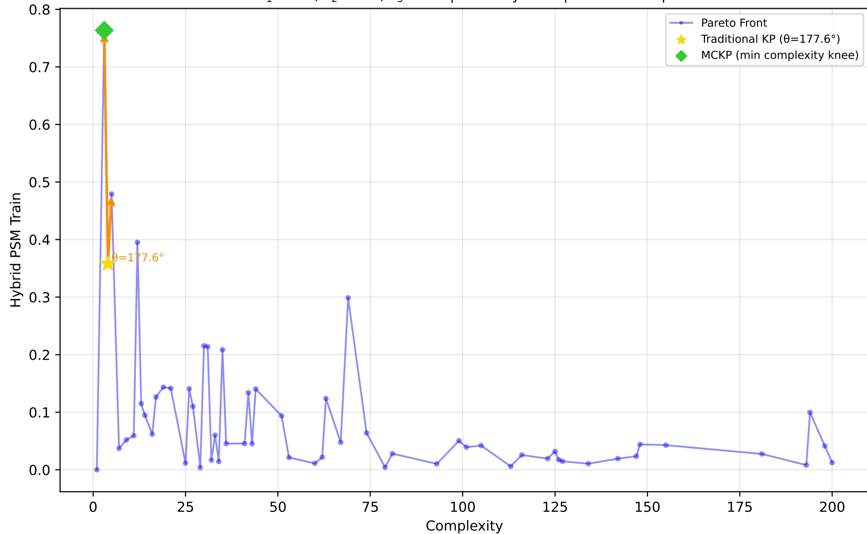
678_visualizing_environmental - Run 8 - MVP - Hybrid PSM Train \lambda_1=0.00, \lambda_2=0.00, \lambda_3=0.10 | Difficulty: 0.21 | Method: mckp
