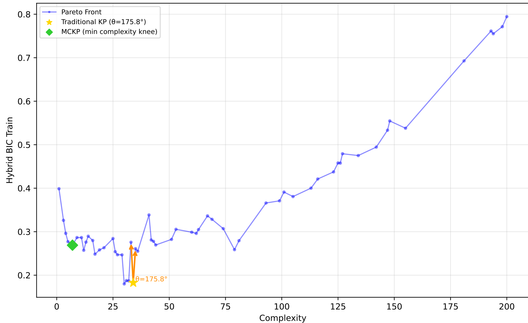
678_visualizing_environmental - Run 8 - SVP - Hybrid BIC Train \lambda_1=0.40, \lambda_2=0.00, \lambda_3=0.00 | Difficulty: 0.21 | Method: mckp
