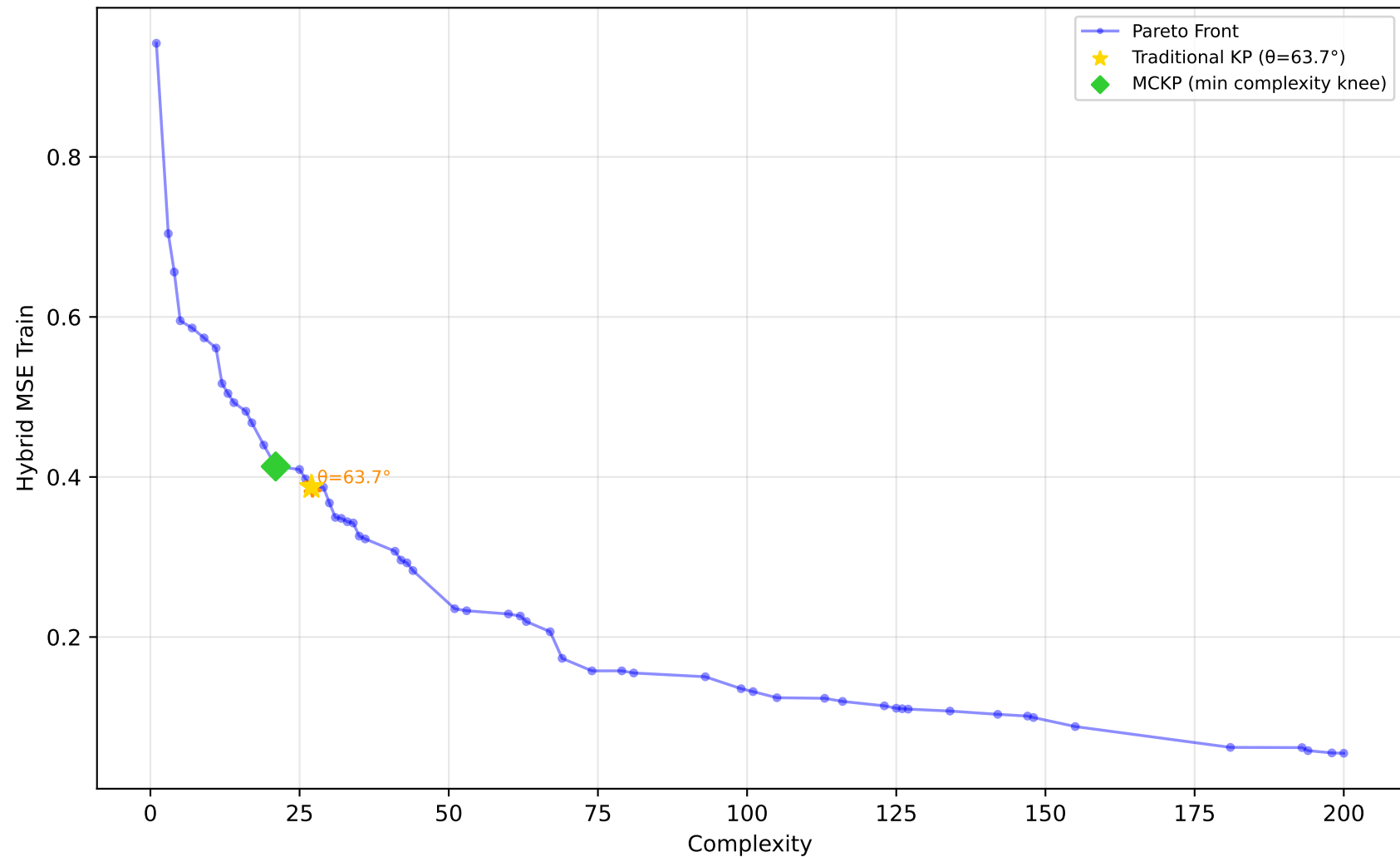
678_visualizing_environmental - Run 8 - SVP - Hybrid MSE Train \lambda_1=0.00, \lambda_2=0.10, \lambda_3=0.20 | Difficulty: 0.21 | Method: mckp
