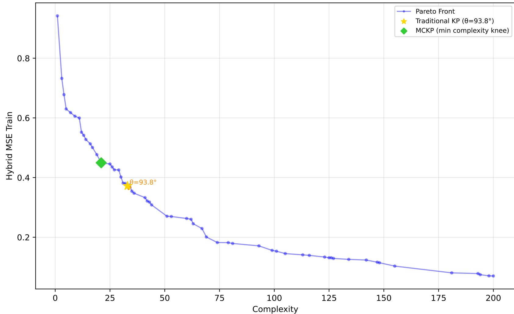
678_visualizing_environmental - Run 8 - SVP - Hybrid MSE Train \lambda_1=0.40, \lambda_2=0.00, \lambda_3=0.00 | Difficulty: 0.21 | Method: mckp
