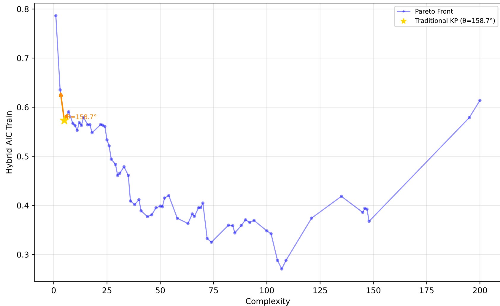
678_visualizing_environmental - Run 9 - MVP - Hybrid AIC Train \lambda_1=0.00, \lambda_2=0.00, \lambda_3=0.10 | Difficulty: 0.41 | Method: mckp
