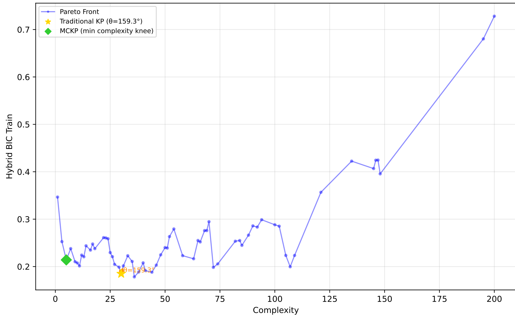
678_visualizing_environmental - Run 9 - MVP - Hybrid BIC Train \lambda_1=0.00, \lambda_2=0.00, \lambda_3=0.10 | Difficulty: 0.41 | Method: mckp
