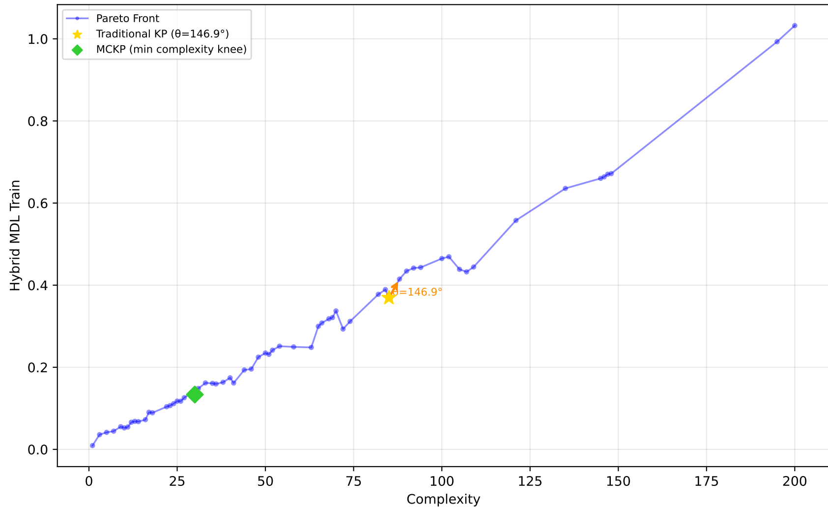
678_visualizing_environmental - Run 9 - MVP - Hybrid MDL Train \lambda_1=0.40 , \lambda_2=0.00 , \lambda_3=0.00 | Difficulty: 0.41 | Method: mckp
