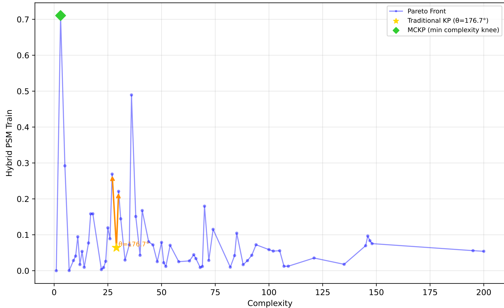
678_visualizing_environmental - Run 9 - MVP - Hybrid PSM Train \lambda_1=0.00, \lambda_2=0.00, \lambda_3=0.10 | Difficulty: 0.41 | Method: mckp
