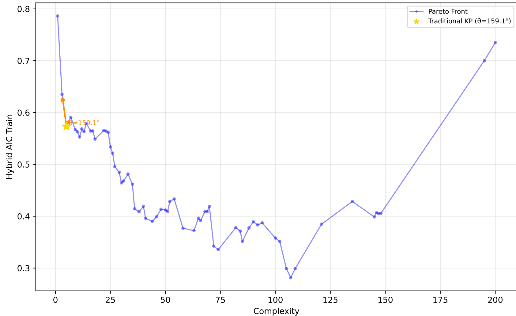
678_visualizing_environmental - Run 9 - SVP - Hybrid AIC Train \lambda_1=0.00, \lambda_2=0.10, \lambda_3=0.20 | Difficulty: 0.41 | Method: mckp
