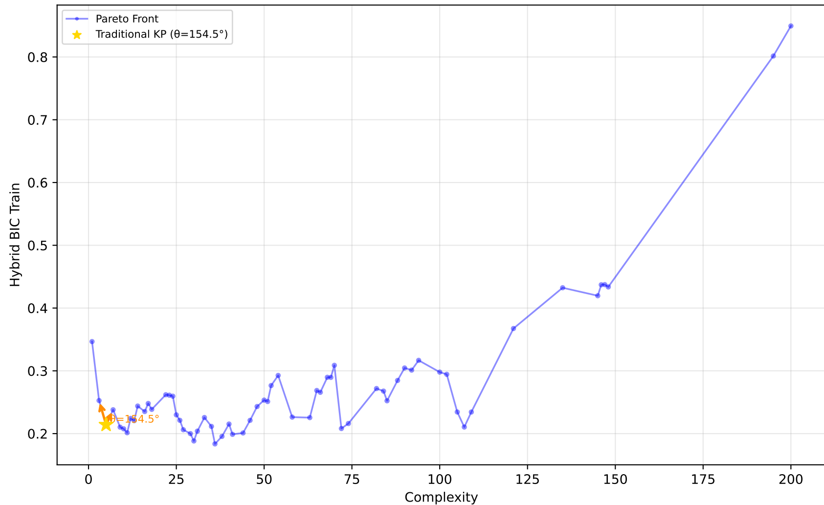
678_visualizing_environmental - Run 9 - SVP - Hybrid BIC Train \lambda_1=0.00, \lambda_2=0.10, \lambda_3=0.20 | Difficulty: 0.41 | Method: mckp
