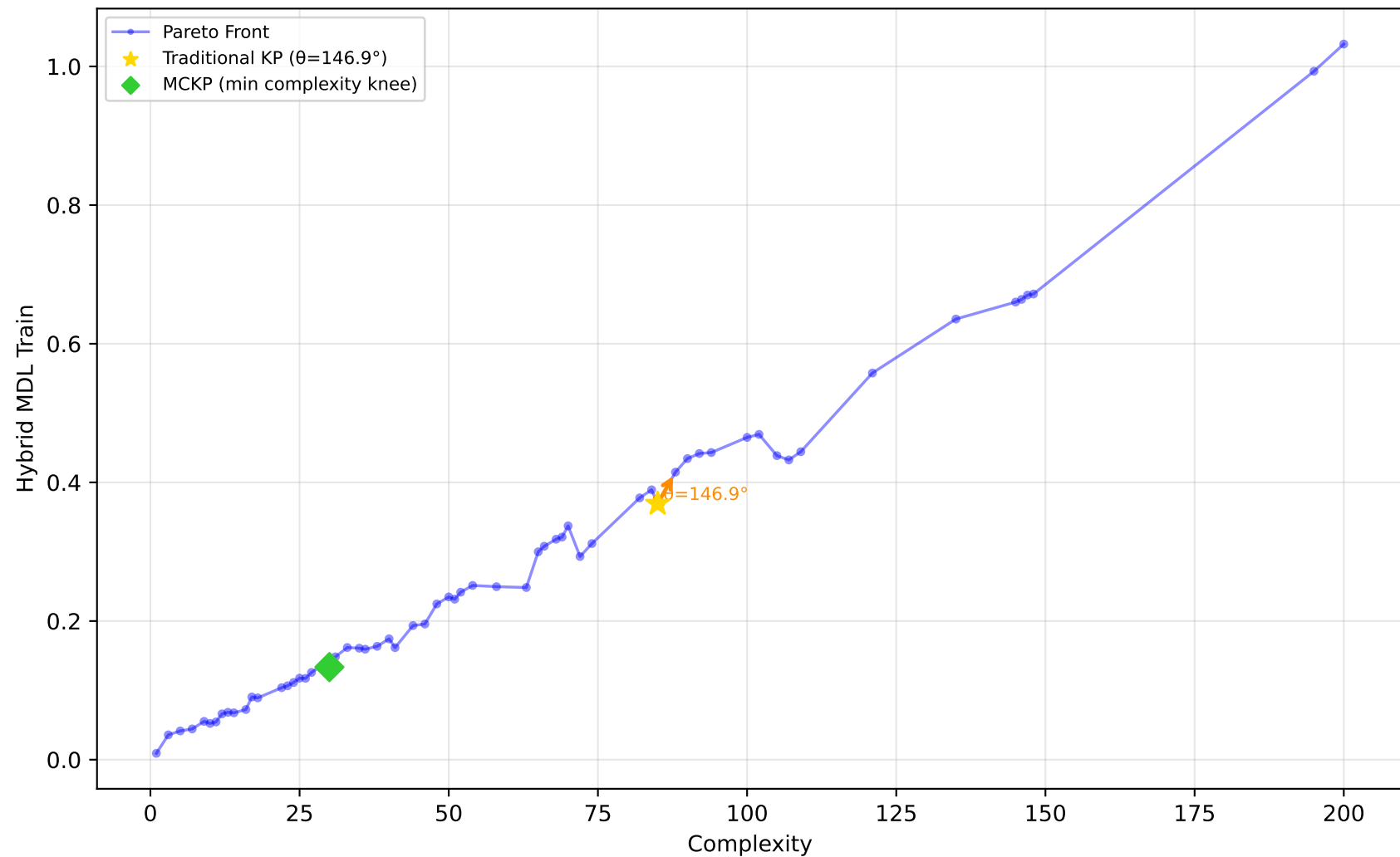
678_visualizing_environmental - Run 9 - SVP - Hybrid MDL Train \lambda_1=0.40 , \lambda_2=0.00 , \lambda_3=0.00 | Difficulty: 0.41 | Method: mckp
