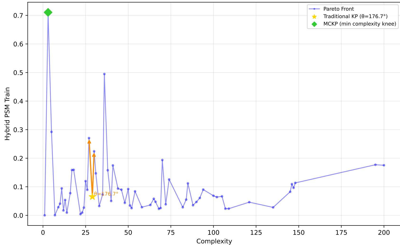
678_visualizing_environmental - Run 9 - SVP - Hybrid PSM Train \lambda_1=0.00, \lambda_2=0.10, \lambda_3=0.20 | Difficulty: 0.41 | Method: mckp
