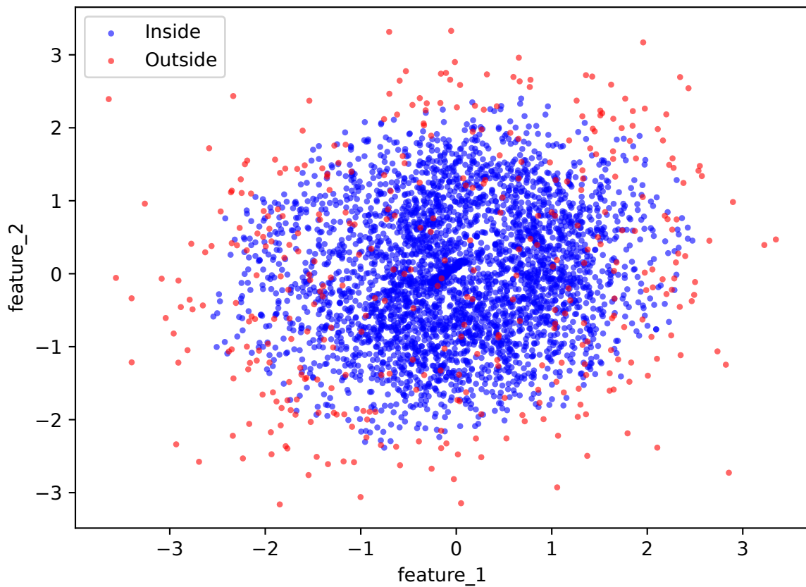
Plot with Bandwidth: 0.34
