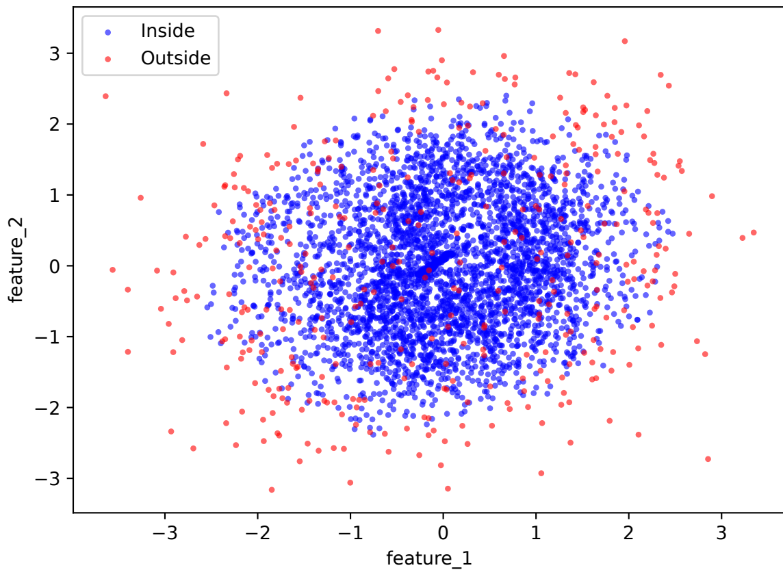
Plot with Bandwidth: 0.36
