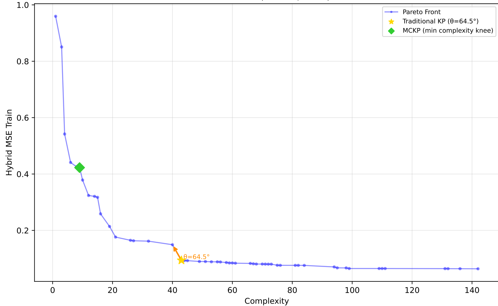
637_fri_c1_500_50 - Run 10 - MVP - Hybrid MSE Train \lambda_1=0.00, \bar{\lambda}_2=0.50, \lambda_3=0.00 | Difficulty: 1.00 | Method: hmr
