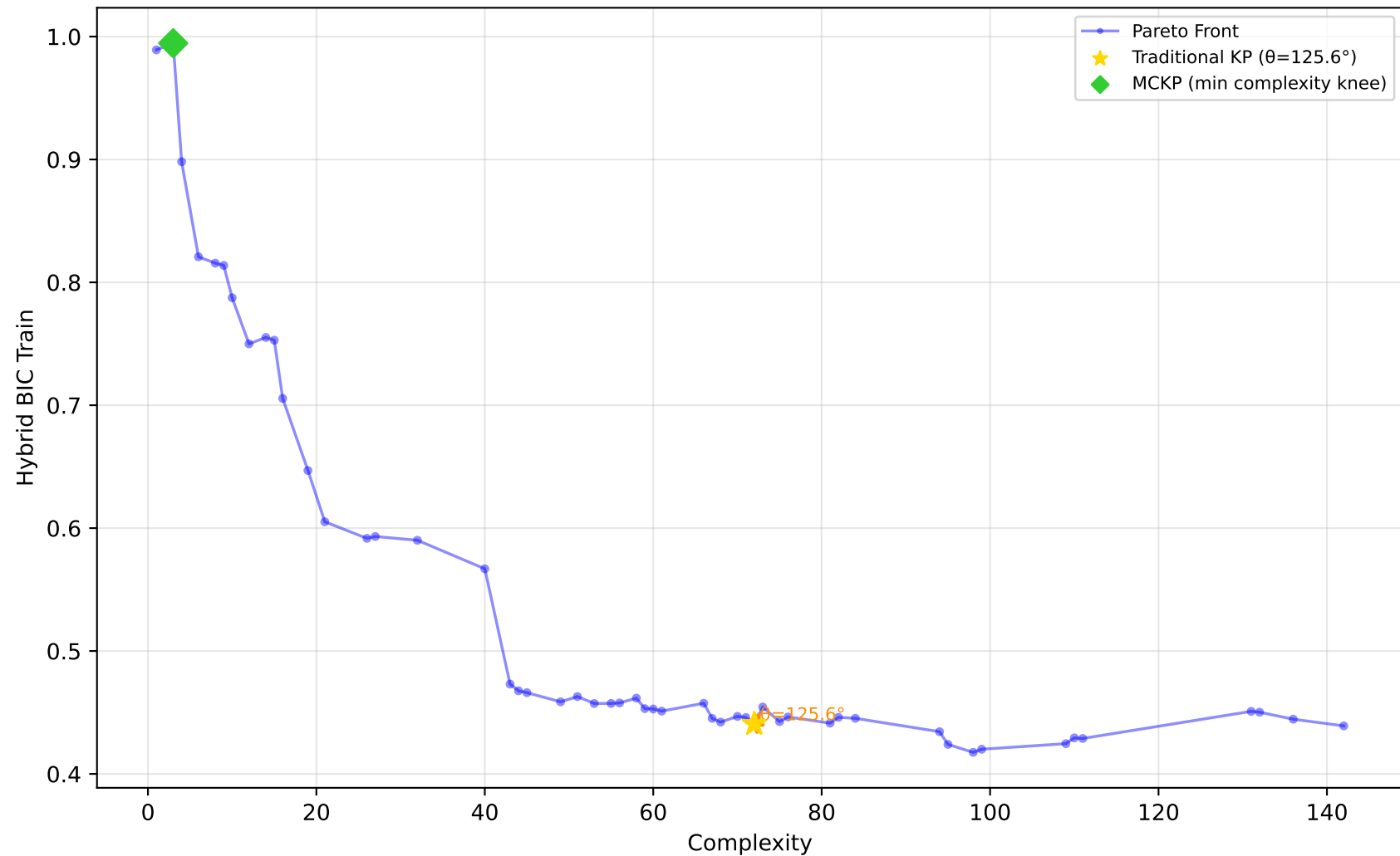
637_fri_c1_500_50 - Run 10 - SVP - Hybrid BIC Train \lambda_1=0.10, \lambda_2=0.00, \lambda_3=0.20 | Difficulty: 1.00 | Method: hmr
