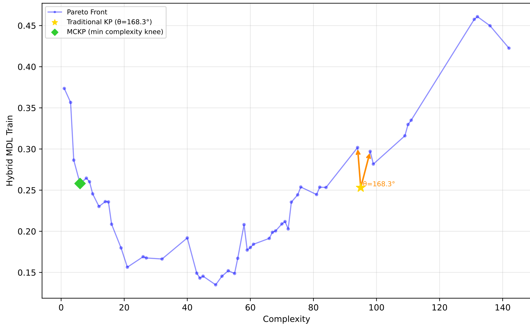
637_fri_c1_500_50 - Run 10 - SVP - Hybrid MDL Train \lambda_1=0.00, \lambda_2=0.00, \lambda_3=0.00 | Difficulty: 1.00 | Method: hmr
