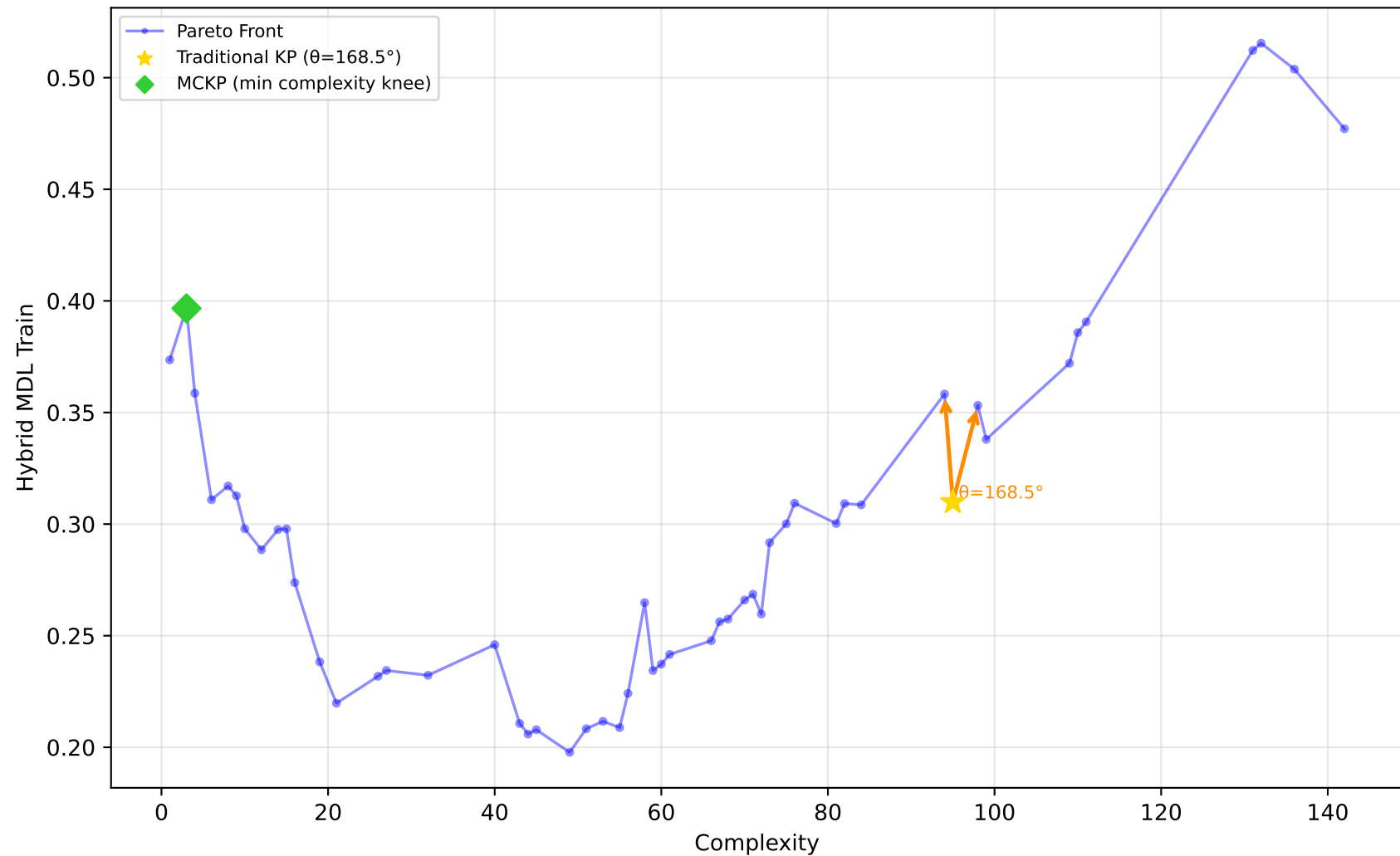
637_fri_c1_500_50 - Run 10 - SVP - Hybrid MDL Train \lambda_1=0.10, \lambda_2=0.00, \lambda_3=0.20 | Difficulty: 1.00 | Method: hmr
