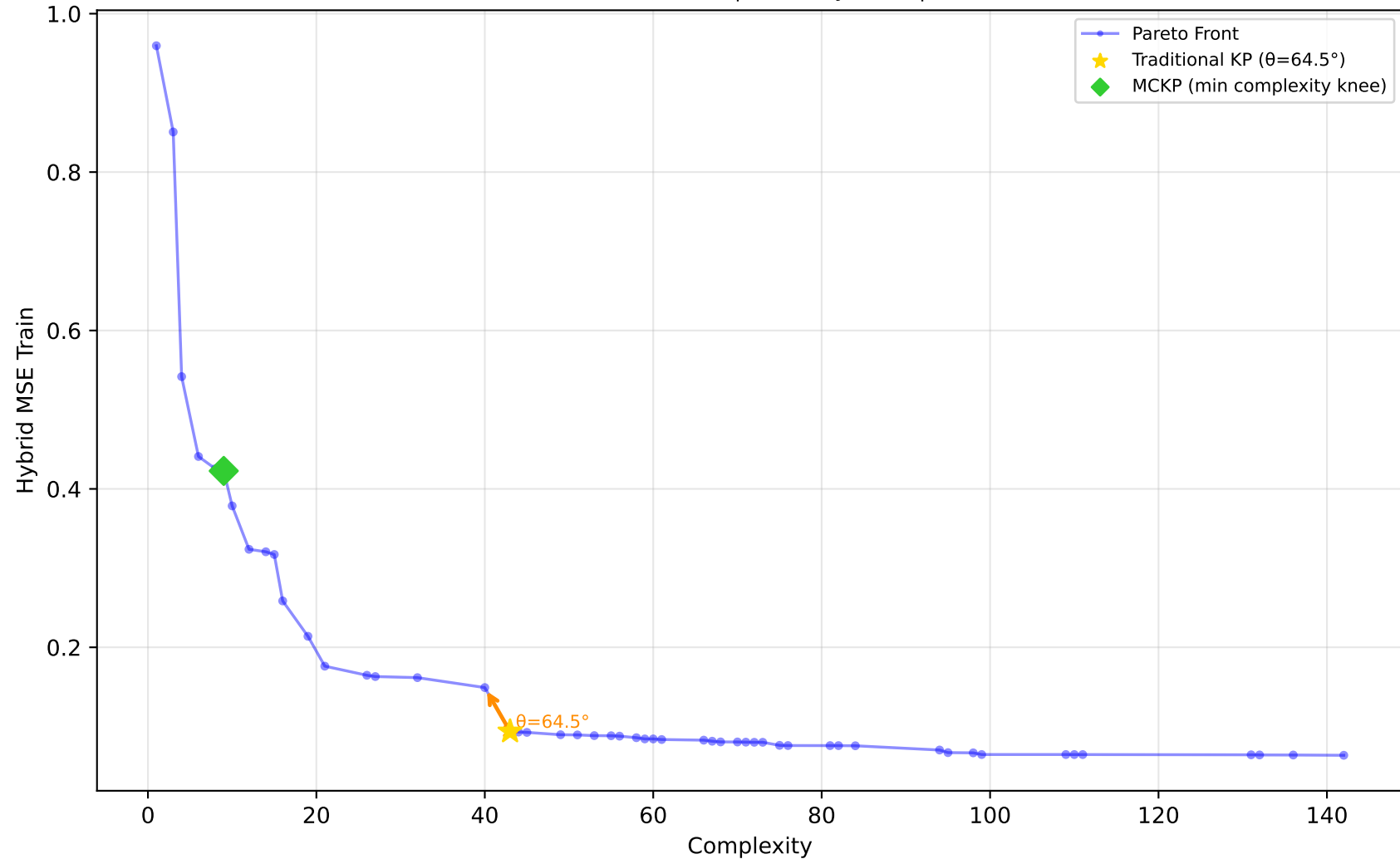
637_fri_c1_500_50 - Run 10 - SVP - Hybrid MSE Train \lambda_1=0.00, \lambda_2=0.00, \lambda_3=0.00 | Difficulty: 1.00 | Method: hmr
