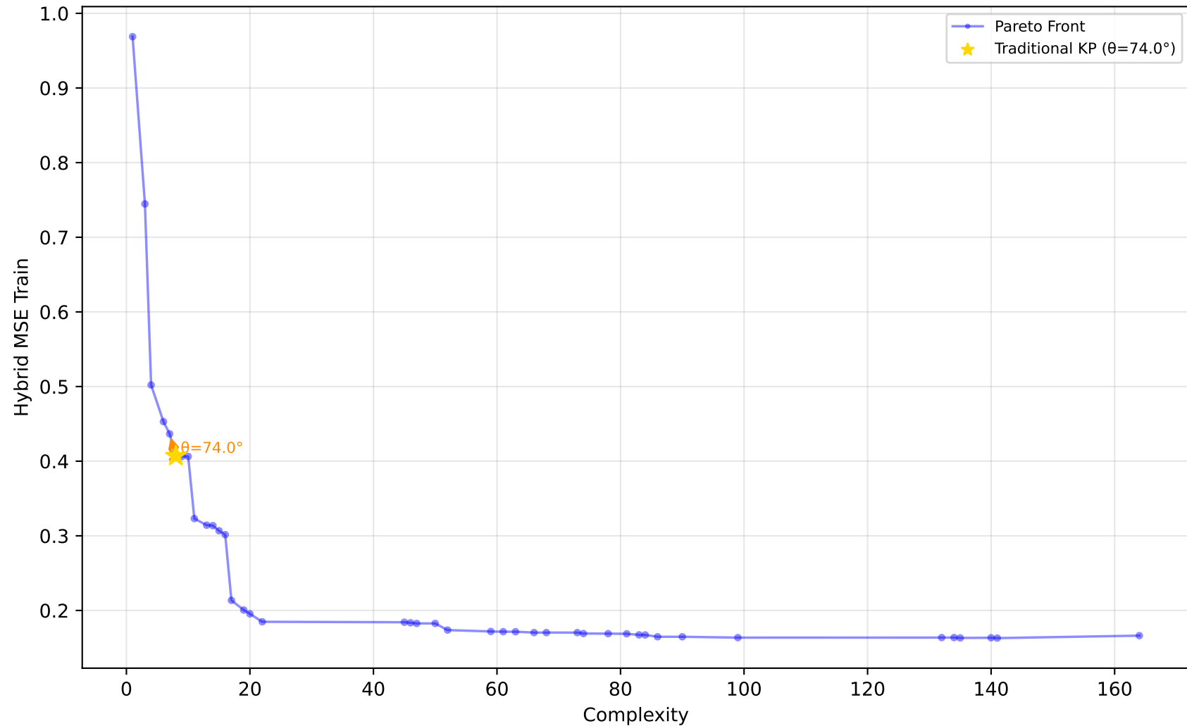
637_fri_c1_500_50 - Run 11 - MVP - Hybrid MSE Train \lambda_1=0.00, \bar{\lambda}_2=0.50, \lambda_3=0.00 | Difficulty: 1.00 | Method: hmr
