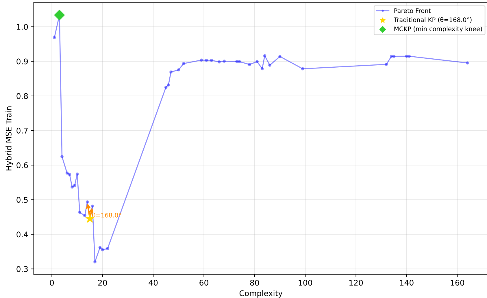
637_fri_c1_500_50 - Run 11 - MVP - Hybrid MSE Train \lambda_1=0.10, \bar{\lambda}_2=0.00, \bar{\lambda}_3=1.00 | Difficulty: 1.00 | Method: hmr
