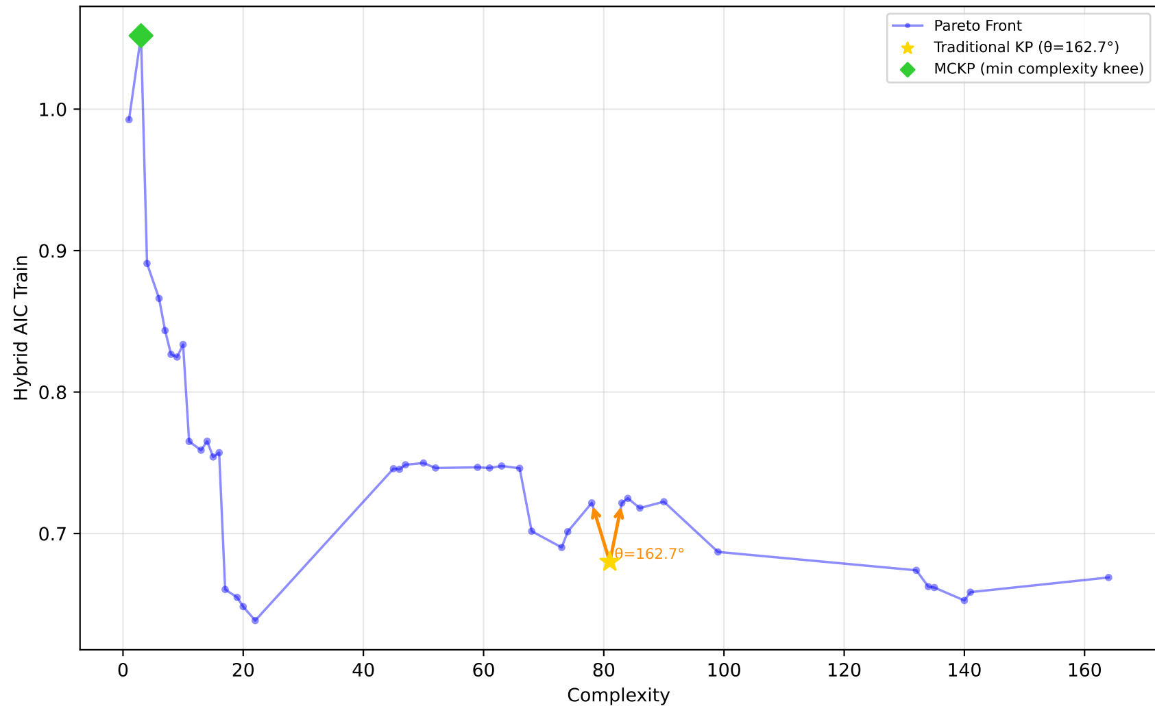
637_fri_c1_500_50 - Run 11 - SVP - Hybrid AIC Train \lambda_1=0.10, \lambda_2=0.00, \lambda_3=0.20 | Difficulty: 1.00 | Method: hmr
