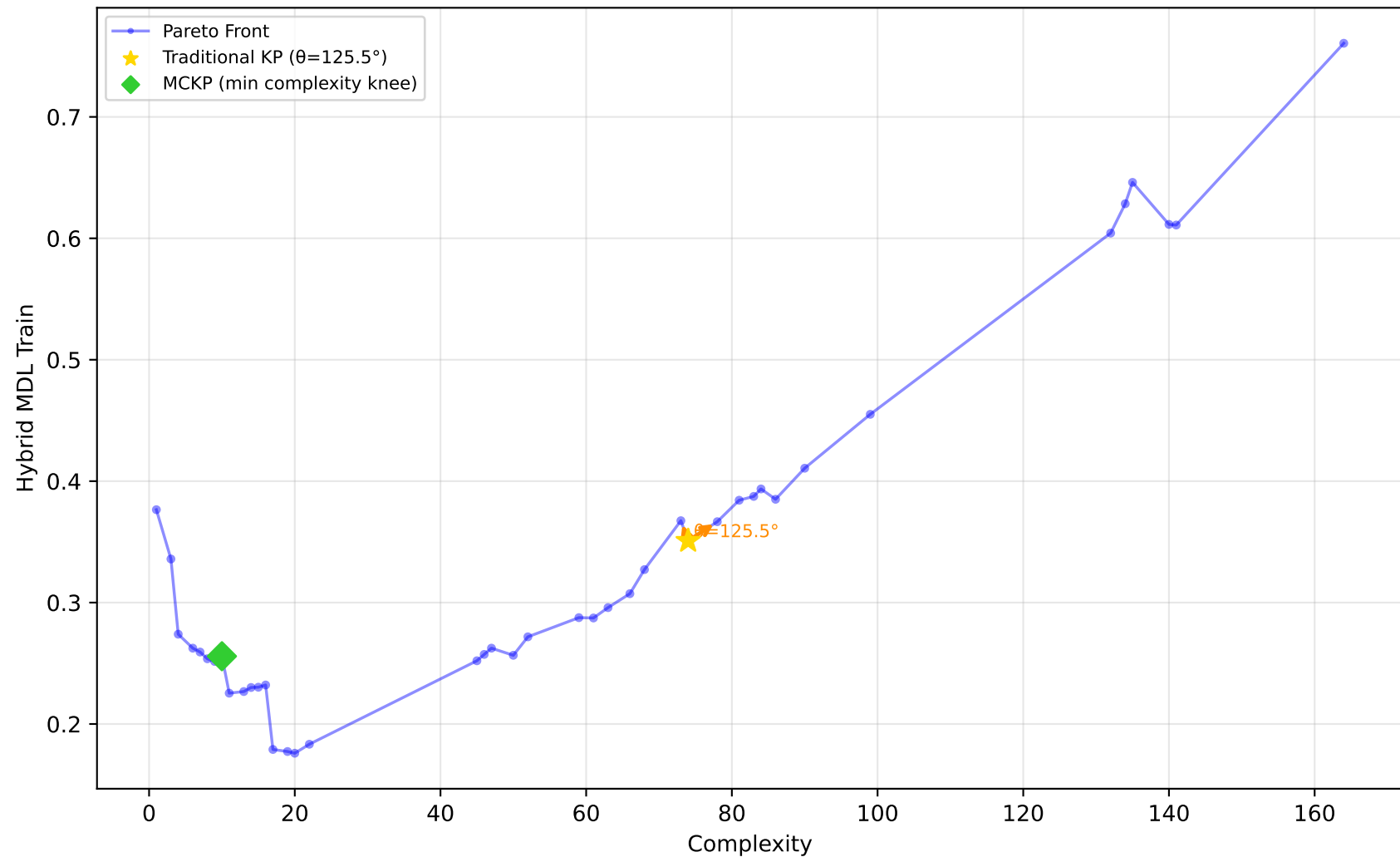
637_fri_c1_500_50 - Run 11 - SVP - Hybrid MDL Train \lambda_1=0.00, \bar{\lambda}_2=0.00, \bar{\lambda}_3=0.00 | Difficulty: 1.00 | Method: hmr
