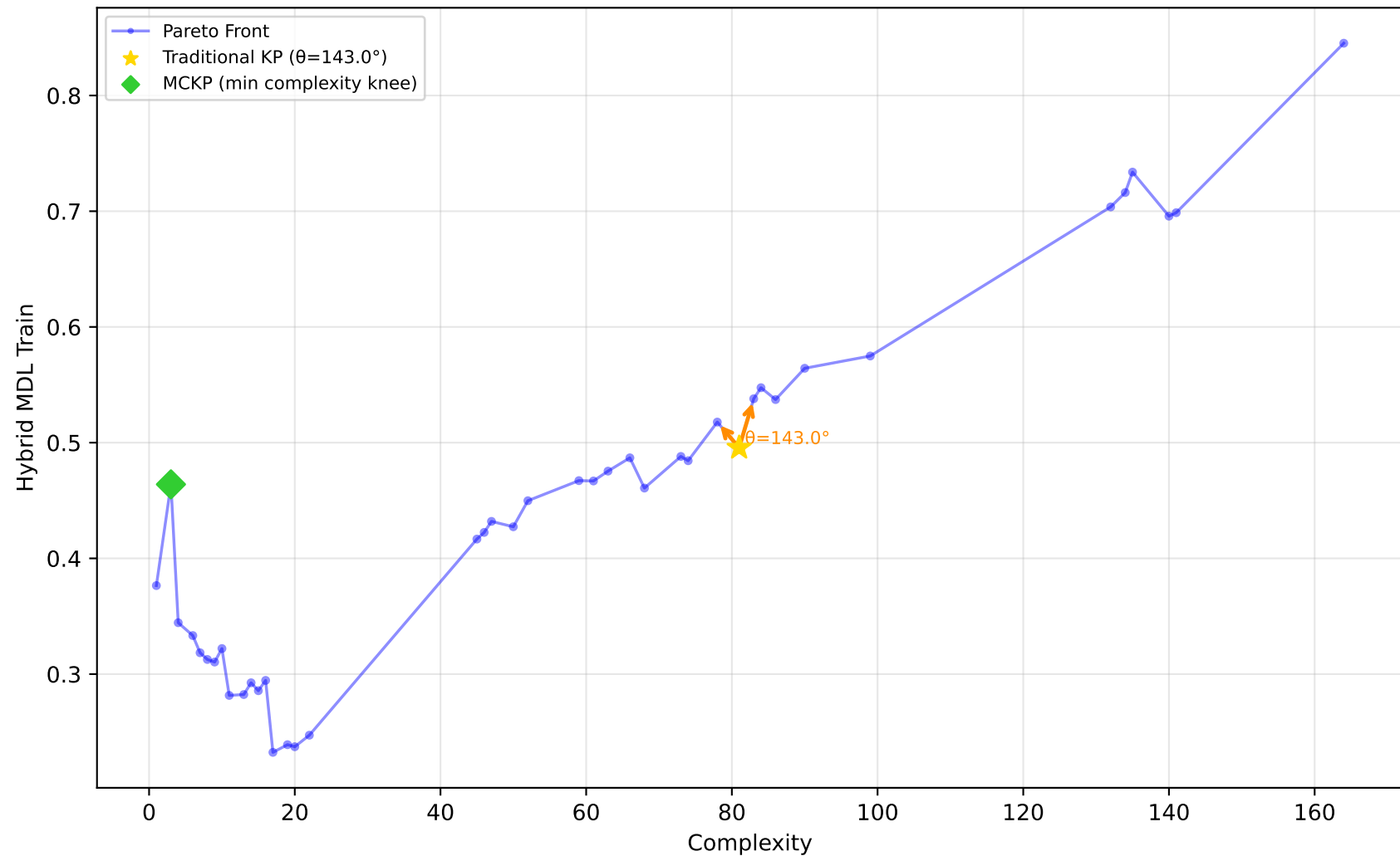
637_fri_c1_500_50 - Run 11 - SVP - Hybrid MDL Train \lambda_1=0.10, \bar{\lambda}_2=0.00, \bar{\lambda}_3=0.20 | Difficulty: 1.00 | Method: hmr
