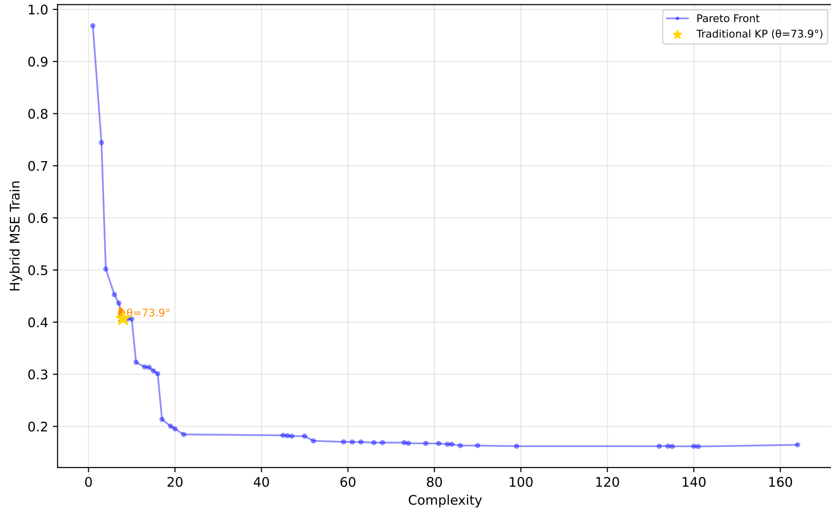
637_fri_c1_500_50 - Run 11 - SVP - Hybrid MSE Train \lambda_1=0.00, \lambda_2=0.00, \lambda_3=0.00 | Difficulty: 1.00 | Method: hmr
