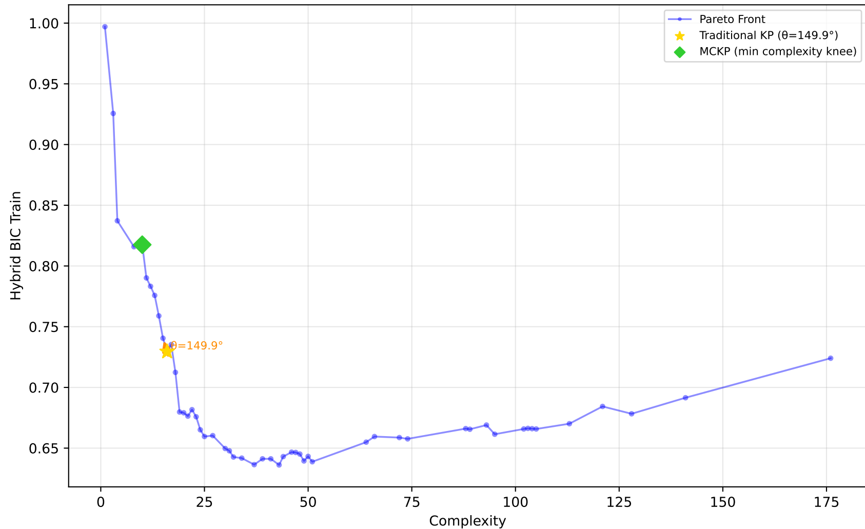
637_fri_c1_500_50 - Run 12 - MVP - Hybrid BIC Train \lambda_1=0.00 , \lambda_2=0.50 , \lambda_3=0.00 | Difficulty: 1.00 | Method: hmr
