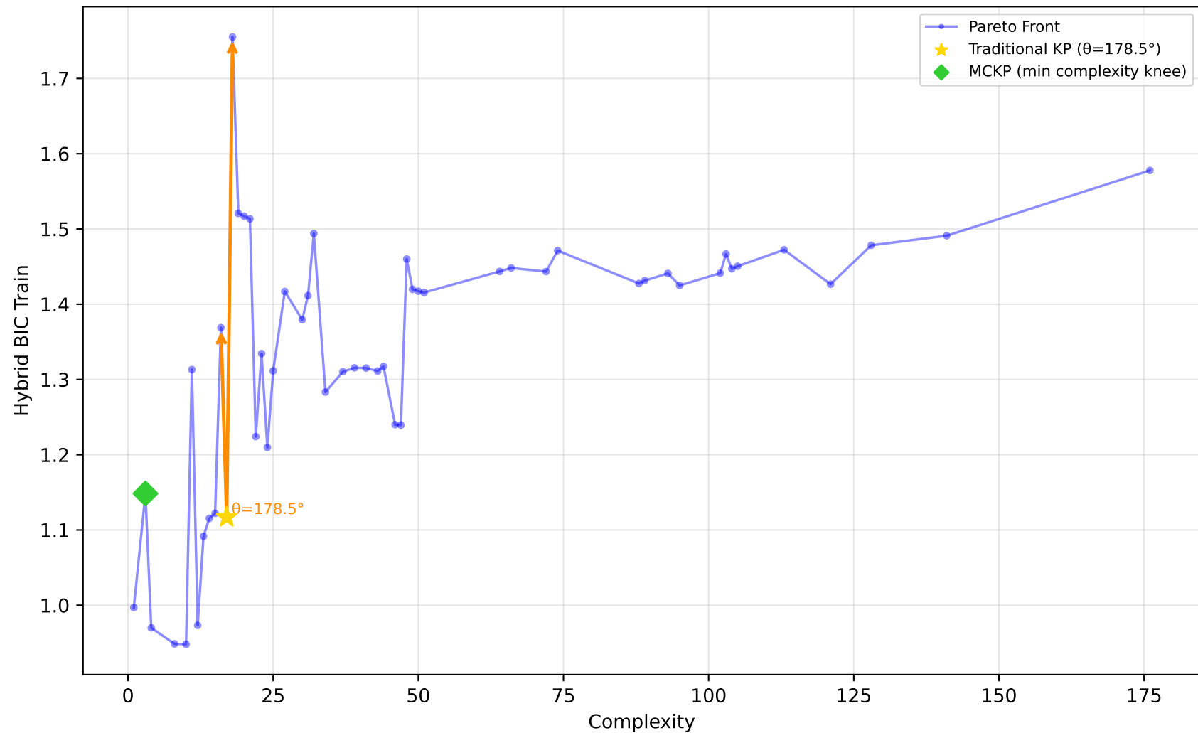
637_fri_c1_500_50 - Run 12 - MVP - Hybrid BIC Train \lambda_1=0.10, \lambda_2=0.00, \lambda_3=1.00 | Difficulty: 1.00 | Method: hmr
