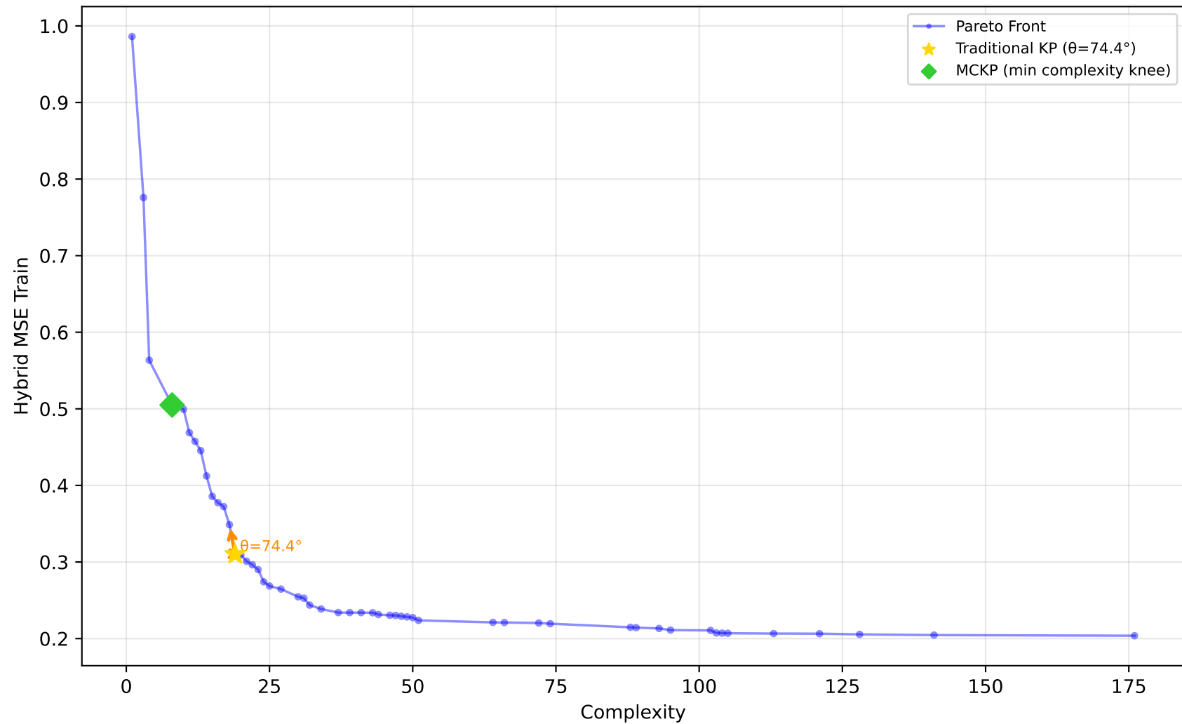
637_fri_c1_500_50 - Run 12 - MVP - Hybrid MSE Train \lambda_1=0.00, \bar{\lambda}_2=0.50, \lambda_3=0.00 | Difficulty: 1.00 | Method: hmr
