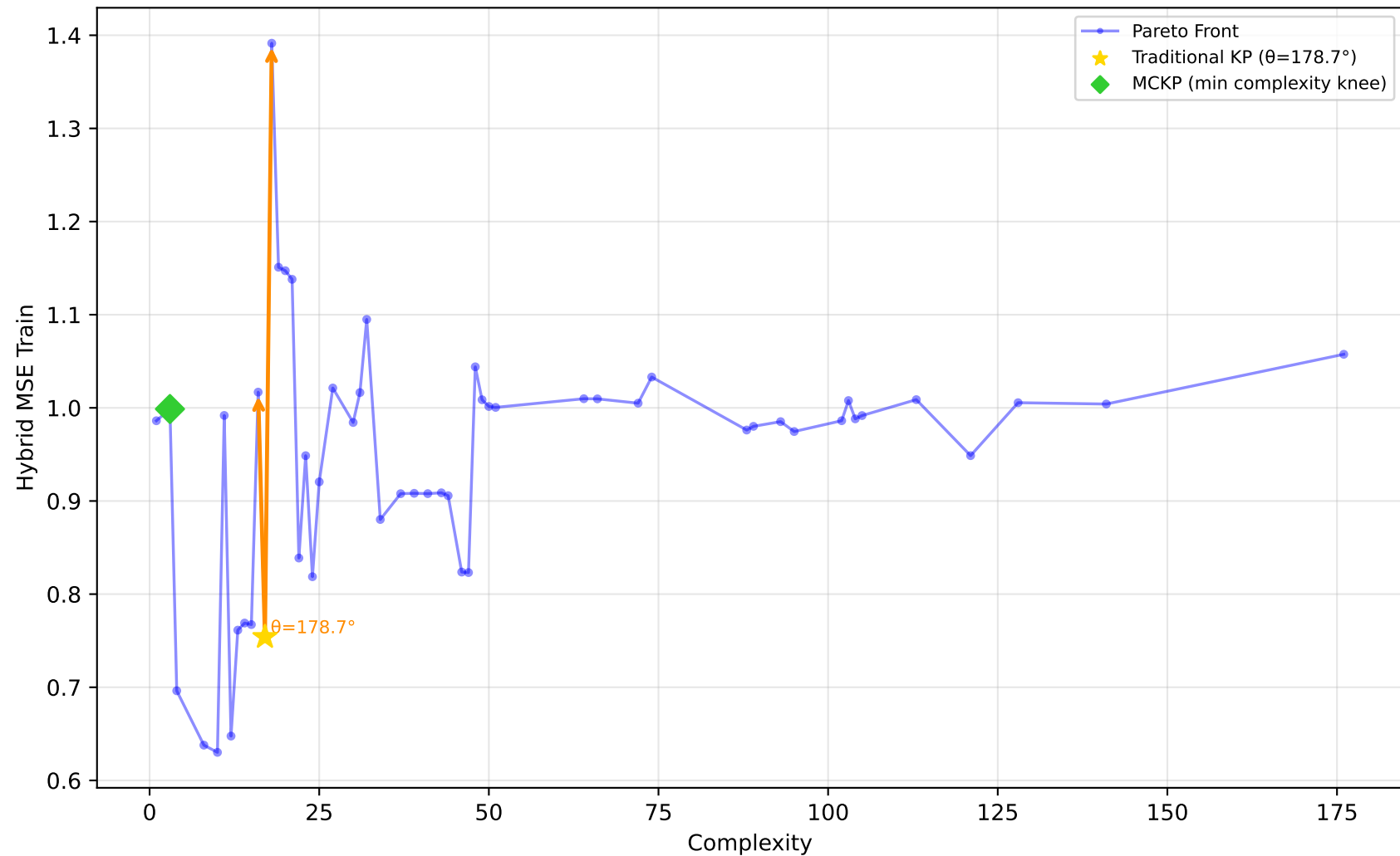
637_fri_c1_500_50 - Run 12 - MVP - Hybrid MSE Train \lambda_1=0.10, \bar{\lambda}_2=0.00, \bar{\lambda}_3=1.00 | Difficulty: 1.00 | Method: hmr
