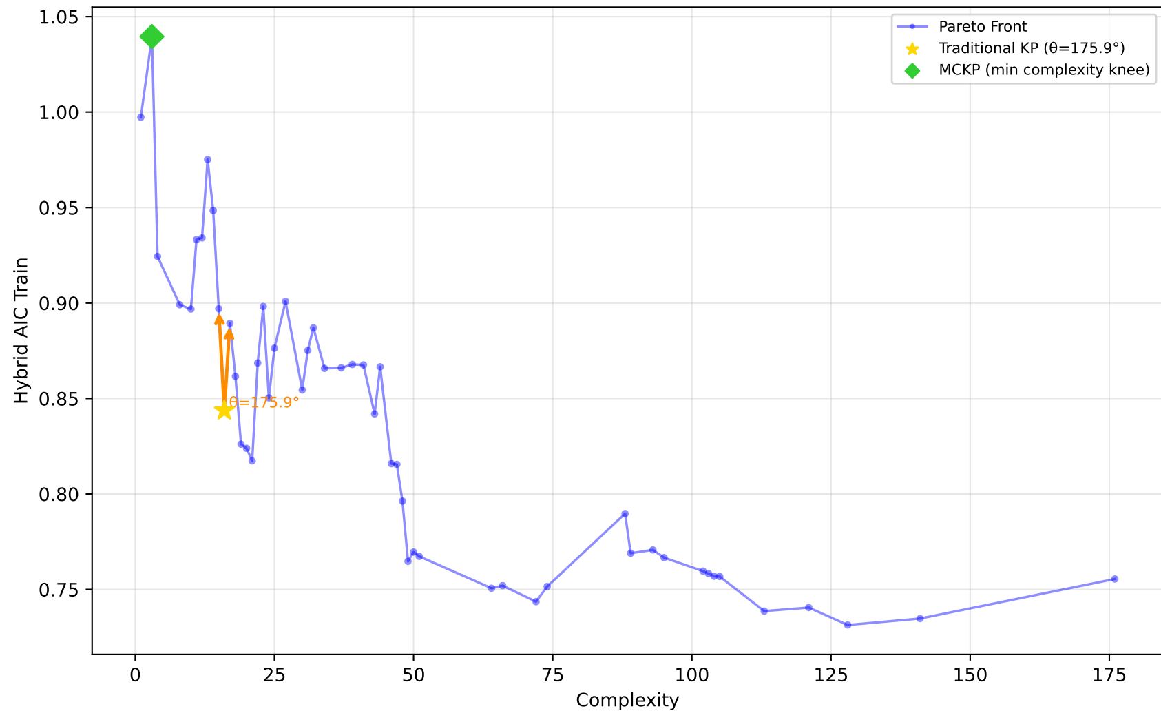
637_fri_c1_500_50 - Run 12 - SVP - Hybrid AIC Train \lambda_1=0.10, \lambda_2=0.00, \lambda_3=0.20 | Difficulty: 1.00 | Method: hmr
