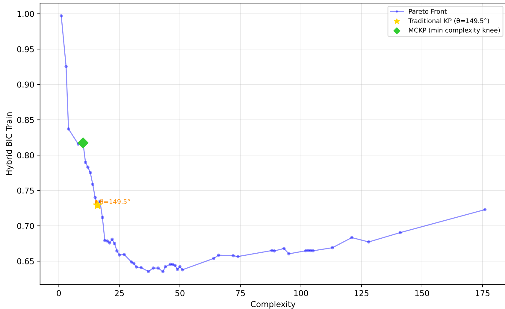
637_fri_c1_500_50 - Run 12 - SVP - Hybrid BIC Train \lambda_1=0.00, \lambda_2=0.00, \lambda_3=0.00 | Difficulty: 1.00 | Method: hmr
