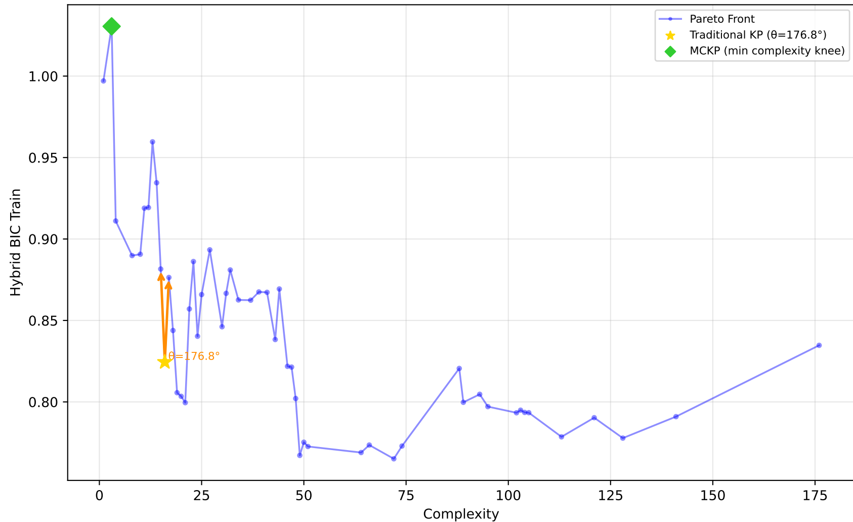
637_fri_c1_500_50 - Run 12 - SVP - Hybrid BIC Train \lambda_1=0.10, \lambda_2=0.00, \lambda_3=0.20 | Difficulty: 1.00 | Method: hmr
