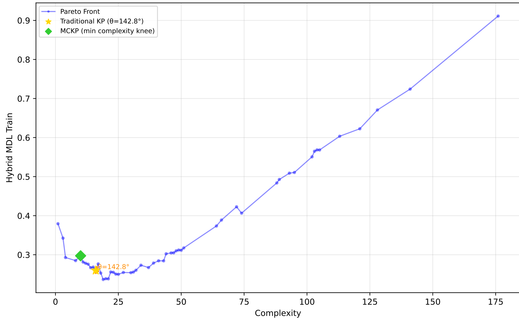
637_fri_c1_500_50 - Run 12 - SVP - Hybrid MDL Train \lambda_1=0.00, \bar{\lambda}_2=0.00, \bar{\lambda}_3=0.00 | Difficulty: 1.00 | Method: hmr
